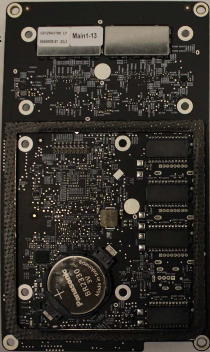
A1470 Main PCB - Back
