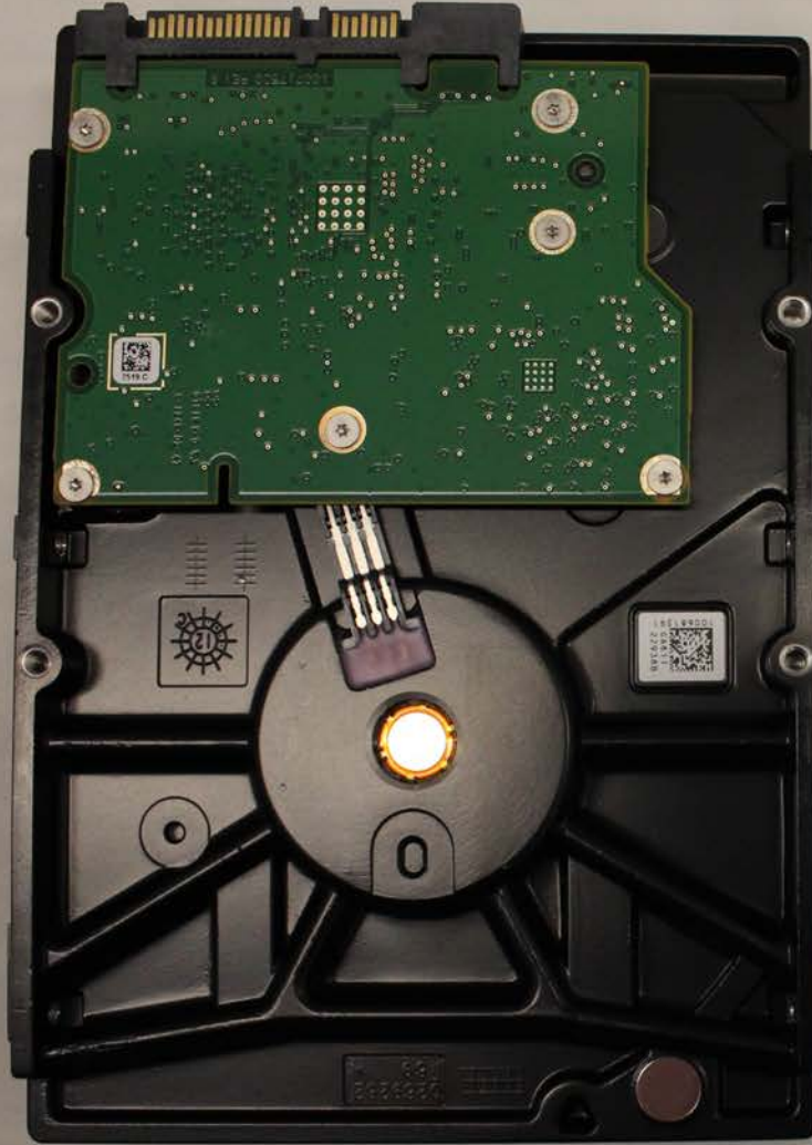
A1470 Hard Disk Drive Bottom side
