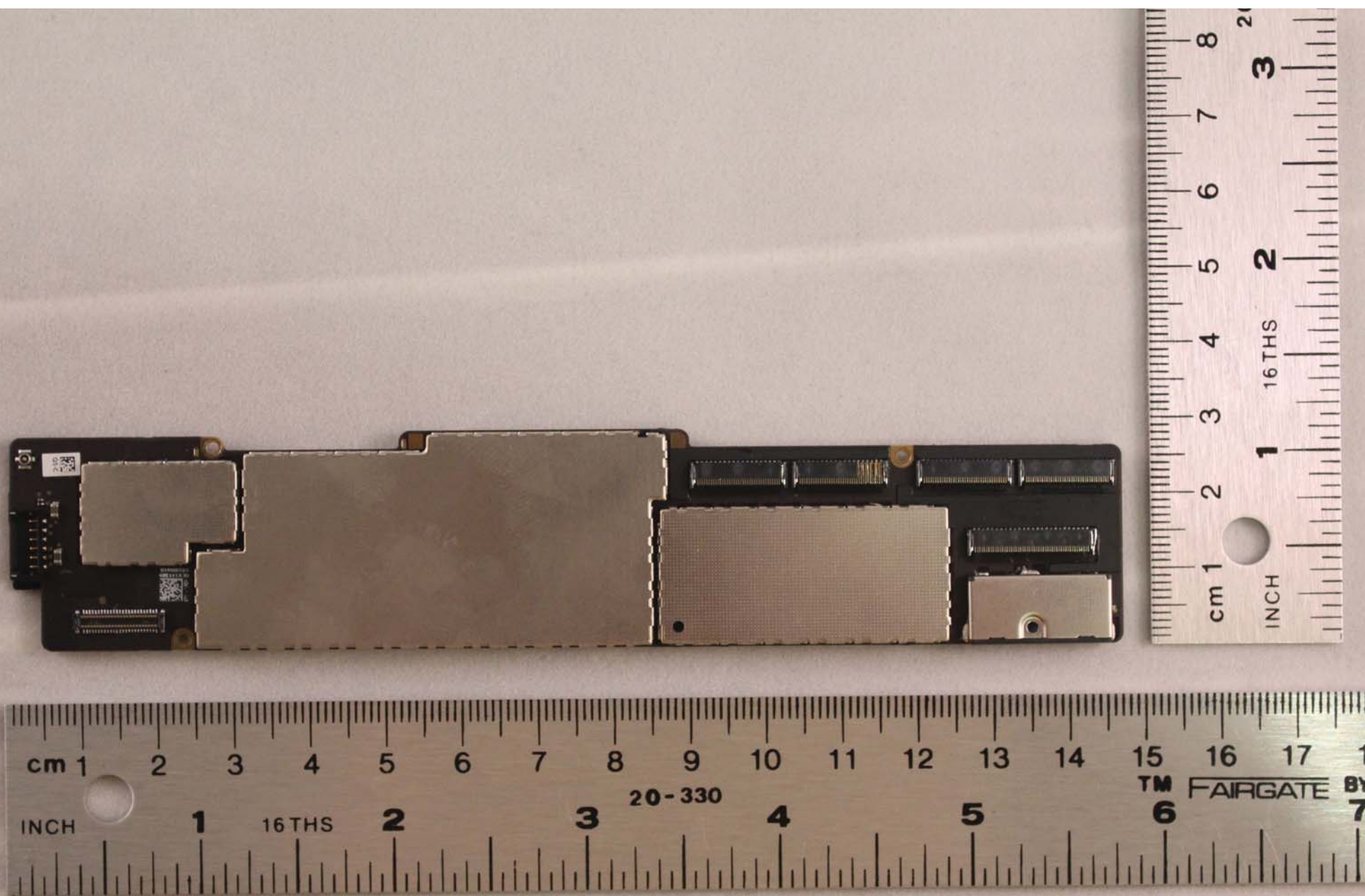
A1403 - Photo 27 Main MLB with shields - Front
