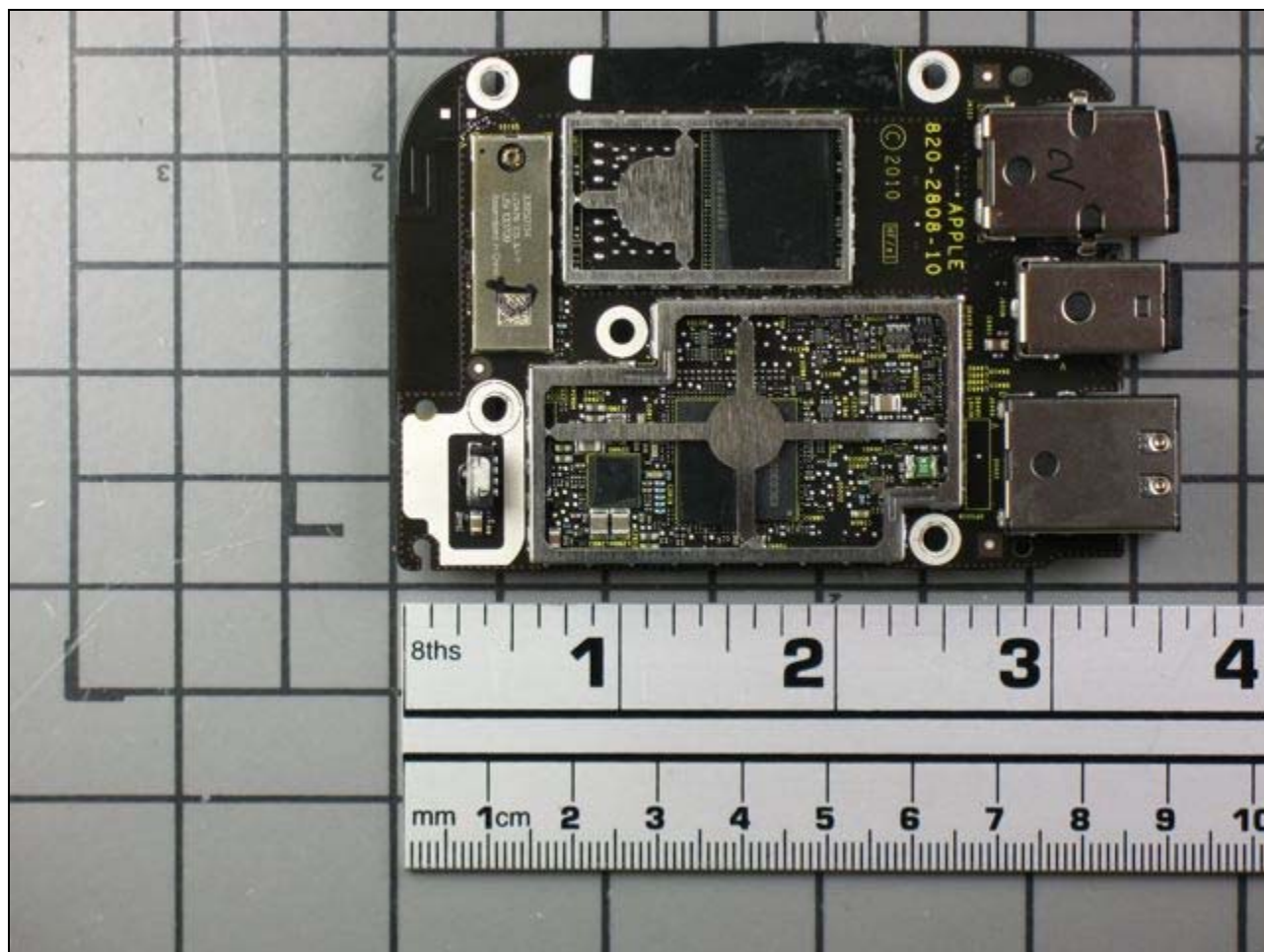
Photograph 1. A1378 PCB Bottom Side
