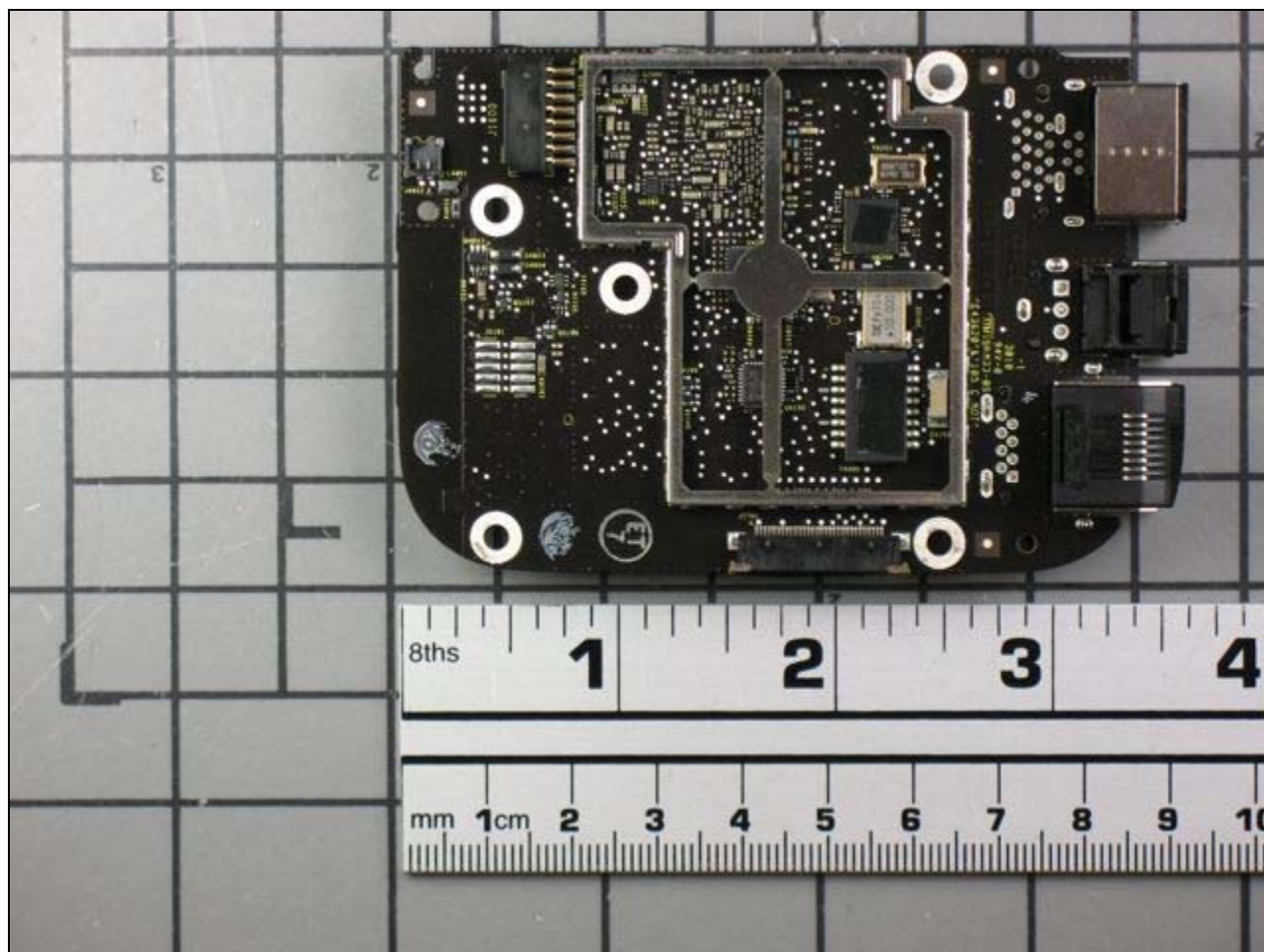
Photograph 2. A1378 PCB Top Side
