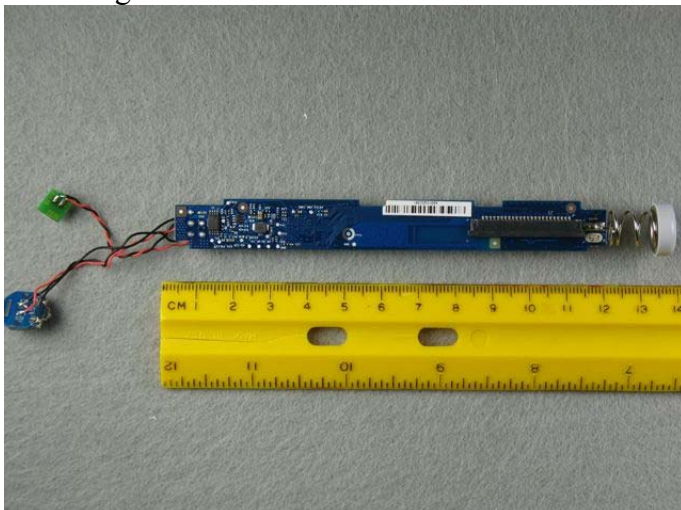
Main Logic Board Bottom Side
