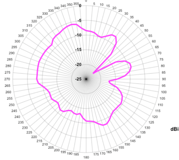
603-1203 Radiation Pattern; Azimuth; 2.45 GHz
