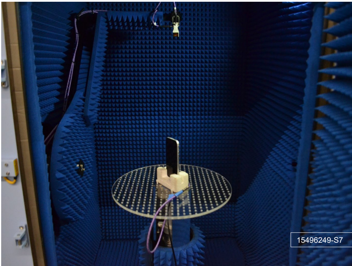
Figure D-3 Radiated power mmW test measurement setup
