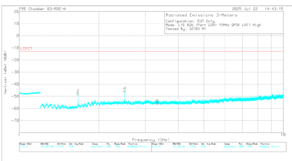
A3525 LTE B26 QPSK High Channel Vertical
