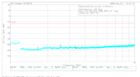
A3257 LTE B26 QPSK High Channel Vertical
