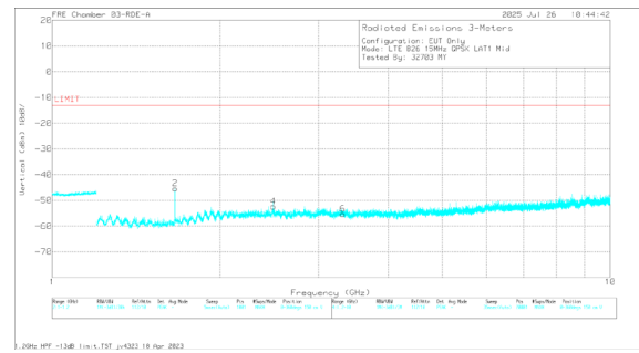
A3526 LTE B26 QPSK Middle Channel Vertical
