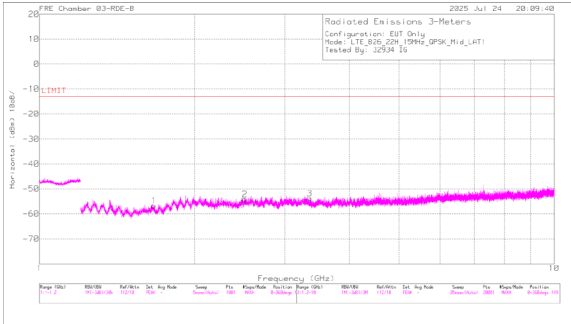
A3527 LTE B26 QPSK Middle Channel Horizontal
