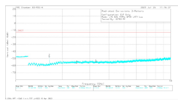
A3526 LTE B26 QPSK Low Channel Vertical
