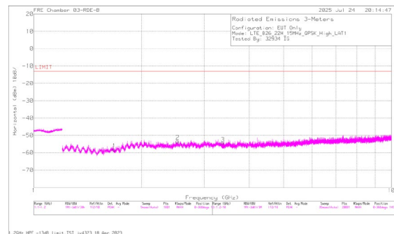
A3527 LTE B26 QPSK High Channel Horizontal
