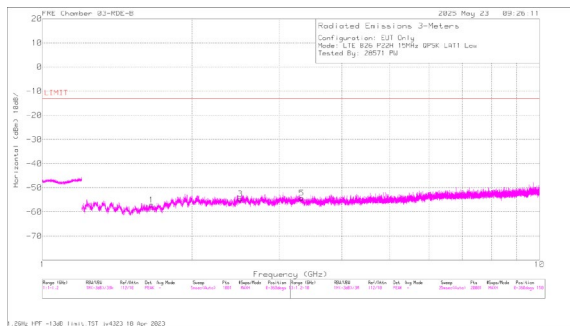
A3257 LTE B26 QPSK Low Channel Horizontal
