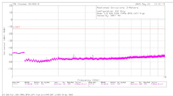
A3257 LTE B26 QPSK High Channel Horizontal
