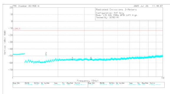
A3526 LTE B26 QPSK High Channel Vertical
