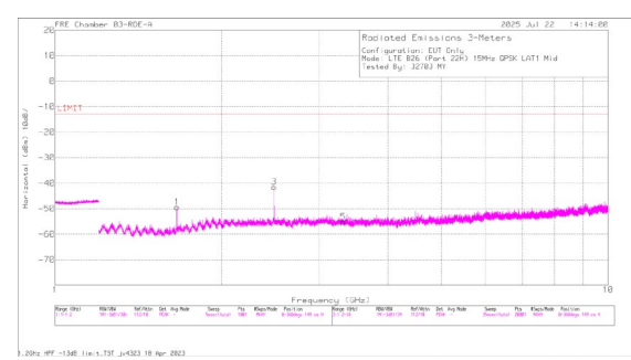
A3525 LTE B26 QPSK Middle Channel Horizontal
