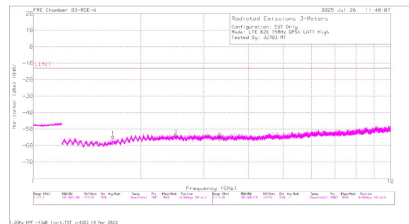
A3526 LTE B26 QPSK High Channel Horizontal
