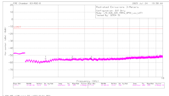
A3527 LTE B26 QPSK Low Channel Horizontal
