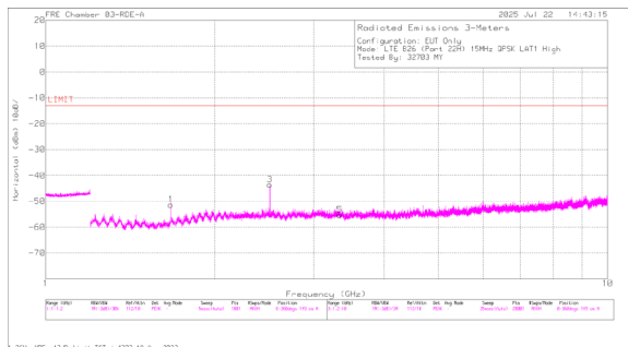
A3525 LTE B26 QPSK High Channel Horizontal
