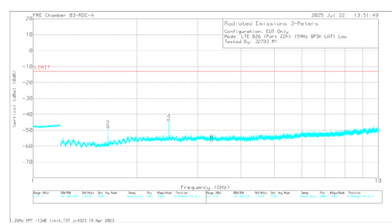
A3525 LTE B26 QPSK Low Channel Vertical
