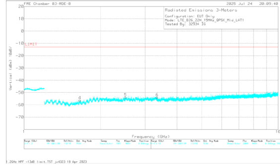
A3527 LTE B26 QPSK Middle Channel Vertical
