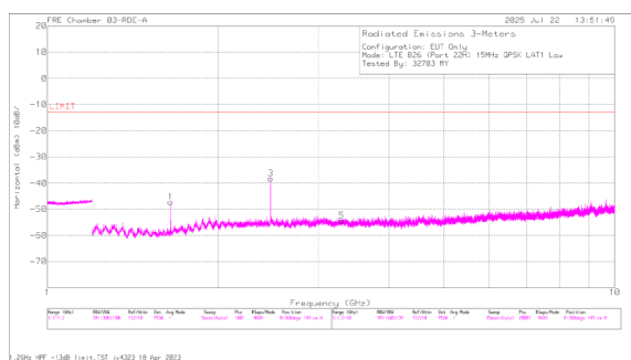
A3525 LTE B26 QPSK Low Channel Horizontal
