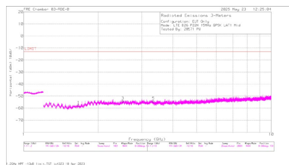
A3257 LTE B26 QPSK Mid Channel Horizontal
