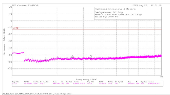
A3257 LTE B26 QPSK High Channel Horizontal
