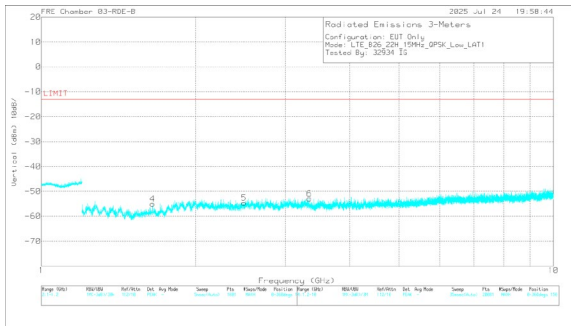
A3527 LTE B26 QPSK Low Channel Vertical
