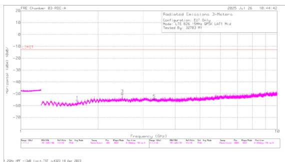
A3526 LTE B26 QPSK Middle Channel Horizontal
