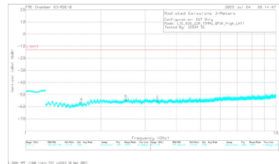
A3527 LTE B26 QPSK High Channel Vertical
