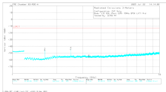
A3525 LTE B26 QPSK Middle Channel Vertical
