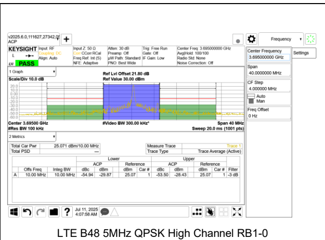
LTE B48 5MHz QPSK High Channel RB1-0
