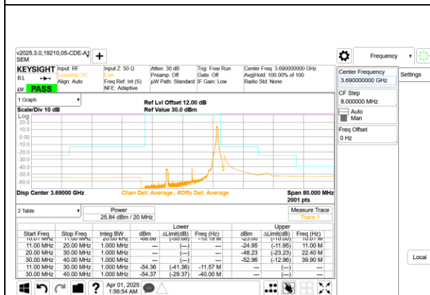
5G NR n48 15MHz BPSK High Channel RB1-37
