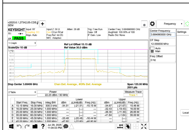
5G NR n48 30MHz BPSK High Channel RB75-0
