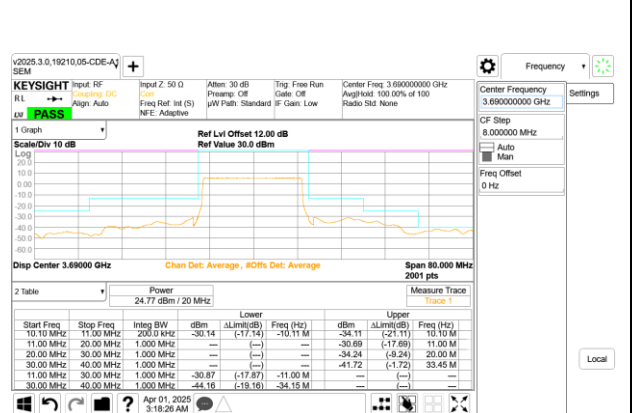
5G NR n48 20MHz BPSK High Channel RB50-0
