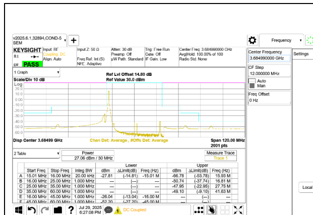
5G NR n48 30MHz BPSK High Channel RB1-0
