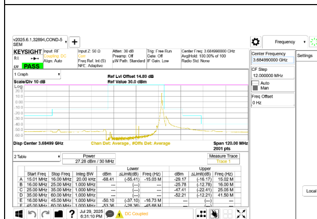
5G NR n48 30MHz BPSK High Channel RB1-77
