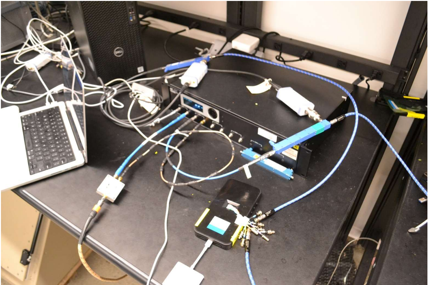
Figure A-1 Default Test Setup for Mode Switch, Band/Antenna Switch with Connection to Router
