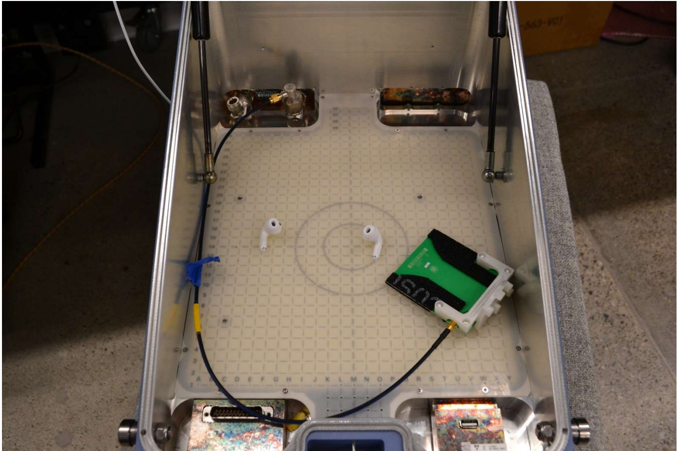
Figure A-4 Bluetooth Conducted Setup in Isolation Box
