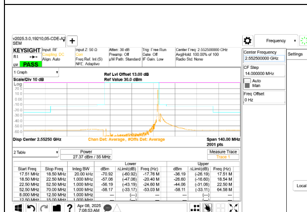
5G NR n7 35MHz BPSK High Channel RB1-187
