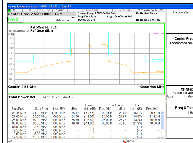
ULCA LTE B7 20MHz + 20MHz QPSK High Ch RB100-0 + RB100-0
