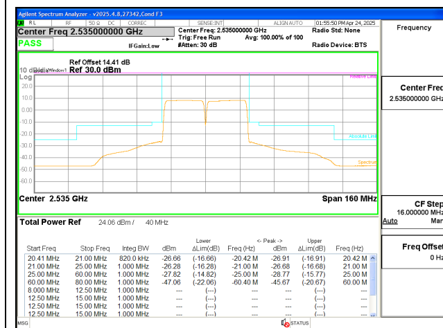
ULCA LTE B7 20MHz + 20MHz QPSK Mid Ch RB100-0 + RB100-0
