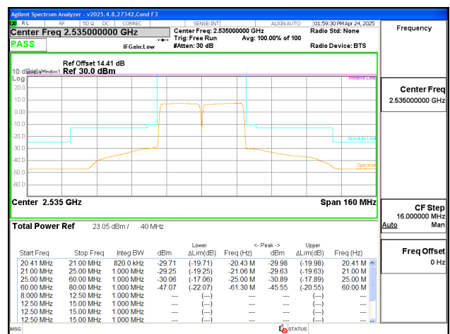
ULCA LTE B7 20MHz + 20MHz 16QAM Mid Ch RB100-0 + RB100-0
