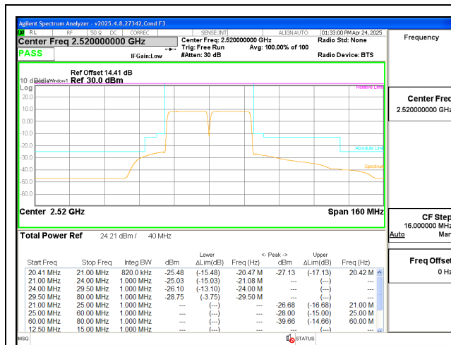
ULCA LTE B7 20MHz + 20MHz QPSK Low Ch RB100-0 + RB100-0
