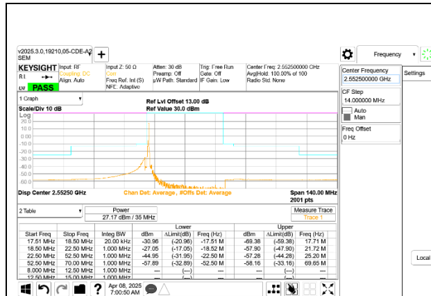
5G NR n7 35MHz BPSK High Channel RB1-0
