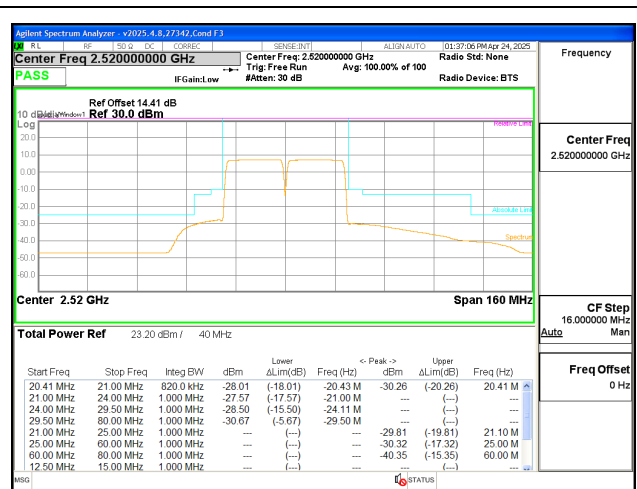
ULCA LTE B7 20MHz + 20MHz 16QAM Low Ch RB100-0 + RB100-0
