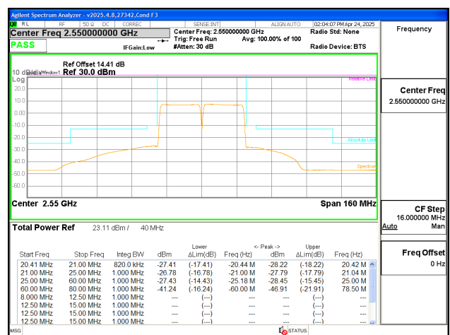
ULCA LTE B7 20MHz + 20MHz 16QAM High Ch RB100-0 + RB100-0
