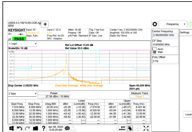
5G NR n7 15MHz BPSK High Channel RB1-0
