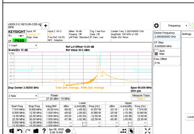
5G NR n7 15MHz BPSK High Channel RB1-78
