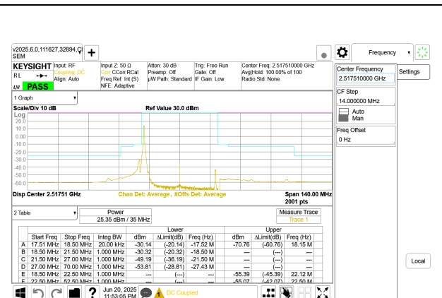
5G NR n41 35MHz BPSK Low Channel RB1-0
