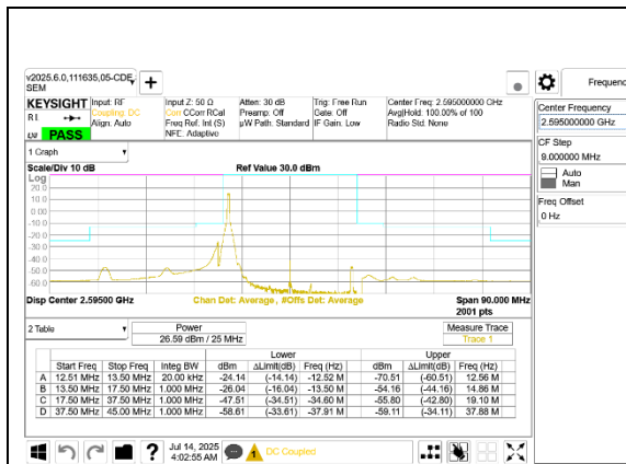
5G NR n41 25MHz BPSK Middle Channel RB1-0
