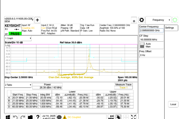
5G NR n41 40MHz BPSK Middle Channel RB1-105
