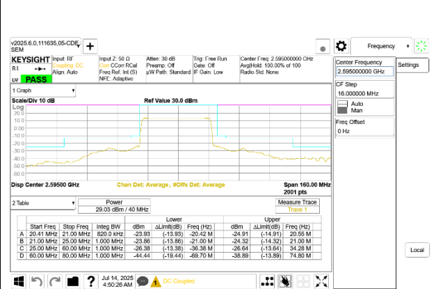
5G NR n41 40MHz BPSK Middle Channel RB100-0
