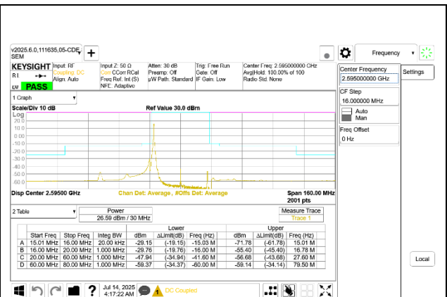
5G NR n41 30MHz BPSK Middle Channel RB1-0
