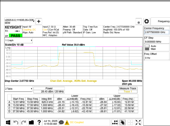
5G NR n41 25MHz BPSK High Channel RB64-0
