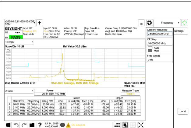
5G NR n41 40MHz BPSK Middle Channel RB1-0
