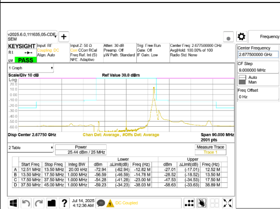
5G NR n41 25MHz BPSK High Channel RB1-64
