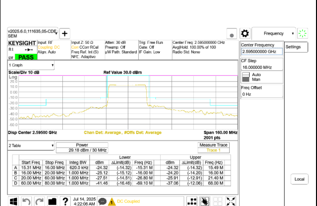
5G NR n41 30MHz BPSK Middle Channel RB75-0
