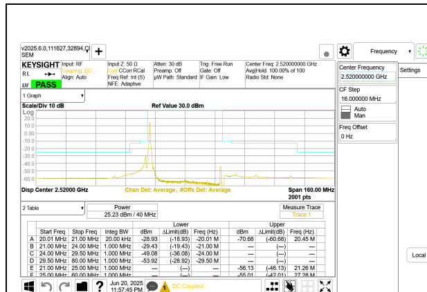
5G NR n41 40MHz BPSK Low Channel RB1-0
