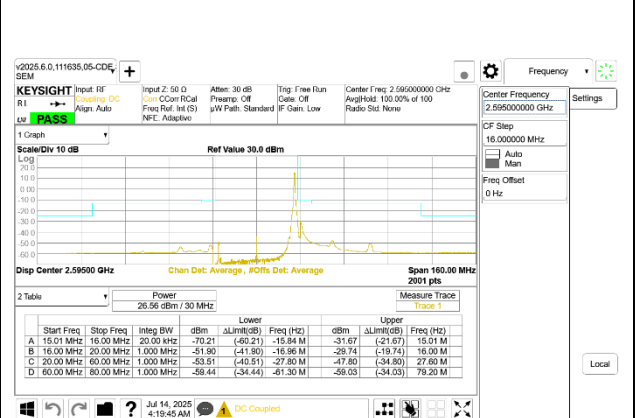
5G NR n41 30MHz BPSK Middle Channel RB1-77
