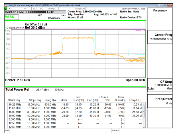
LTE B41 20MHz QPSK High Channel RB100-0
