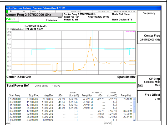
5G NR n41 15MHz BPSK Low Channel RB1-37
