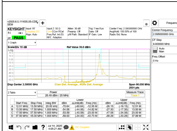
5G NR n41 25MHz BPSK Middle Channel RB1-64
