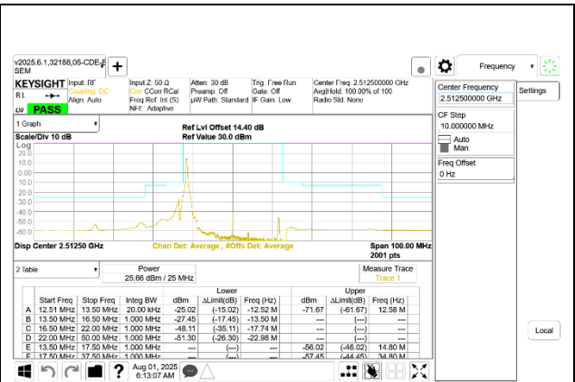
5G NR n41 25MHz BPSK Low Channel RB1-0
