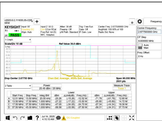
5G NR n41 25MHz BPSK High Channel RB1-0
