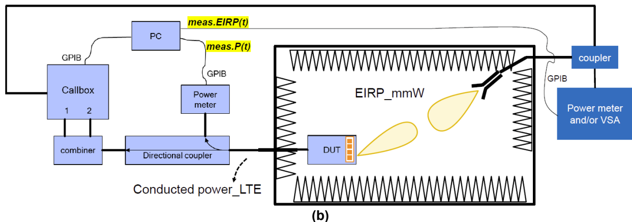
Figure 10-1 mmW NR radiated power measurement setup
