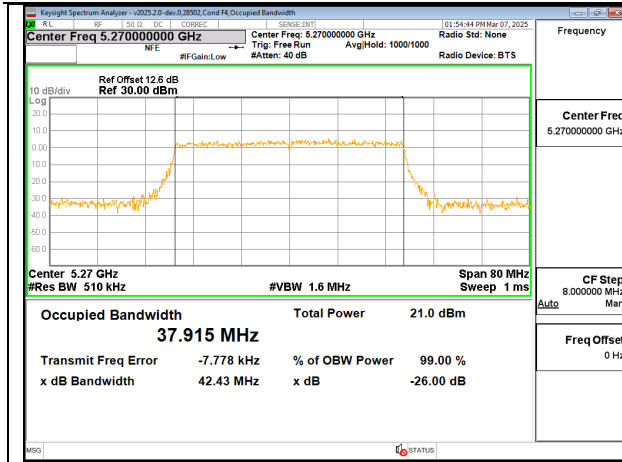
40MHz - Mid Channel – SU (UNII-2A) – ANT 5
