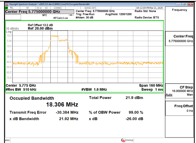
80MHz - Mid Channel – 106T RU53 (UNII-3) – ANT 6
