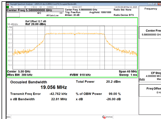
20MHz - Mid Channel – SU (UNII-2C) – ANT 5
