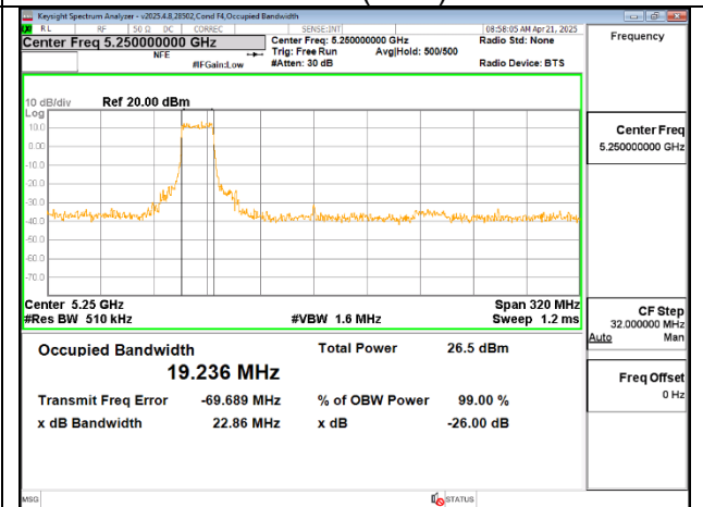
160MHz - Mid Channel – 242T RU61 (UNII-1) – ANT 5 (FCC)
