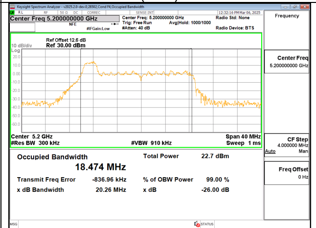
20MHz - Mid Channel – 26T RU0 (UNII-1) – ANT 5 (FCC)
