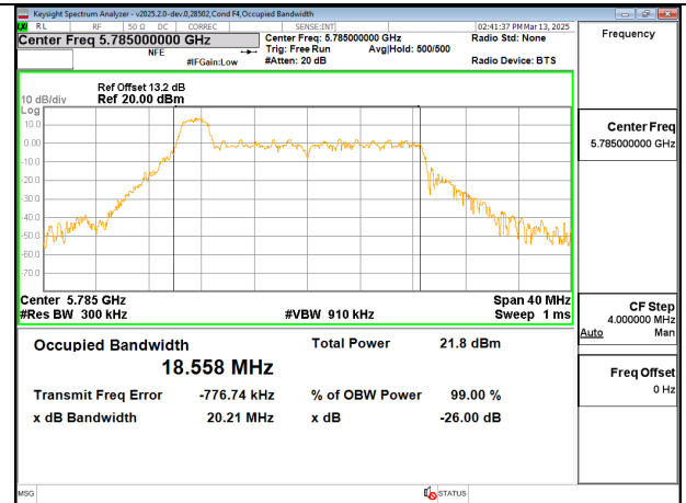
20MHz - Mid Channel – 26T RU0 (UNII-3) – ANT 6
