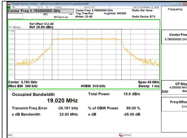
20MHz - Mid Channel – SU (UNII-3) – ANT 6
