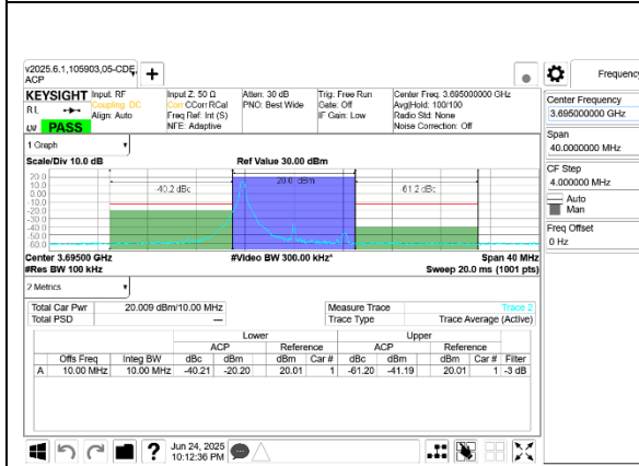
5G NR n48 10MHz QPSK High Channel RB1-0 Port B
