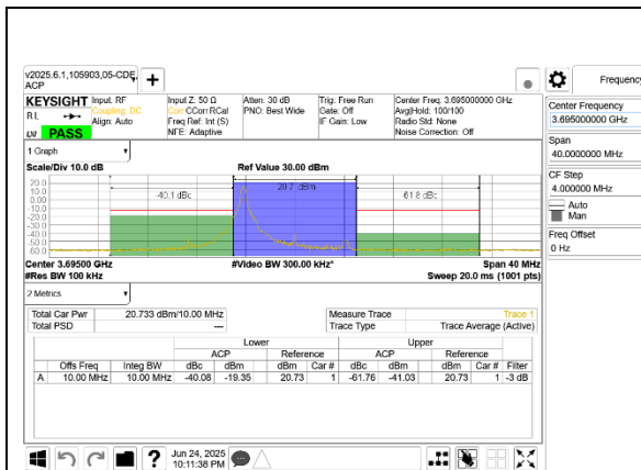
5G NR n48 10MHz QPSK High Channel RB1-0 Port A
