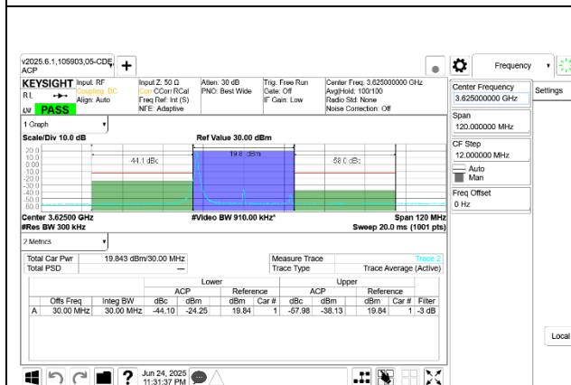
5G NR n48 30MHz QPSK Mid Channel RB1-0 Port B
