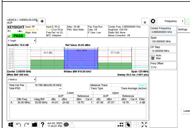
5G NR n48 30MHz QPSK High Channel RB1-0 Port B
