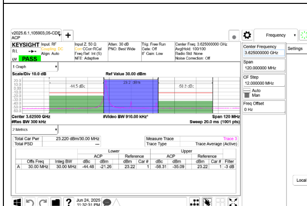
5G NR n48 30MHz QPSK Mid Channel RB1-0 Port A+B
