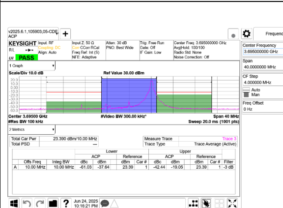
5G NR n48 10MHz QPSK High Channel RB1-23 Port A+B
