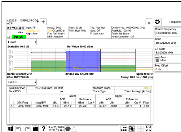
5G NR n48 20MHz QPSK High Channel RB1-0 Port A
