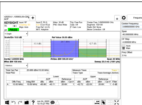
5G NR n48 10MHz QPSK High Channel RB1-23 Port A, ID: 27957
