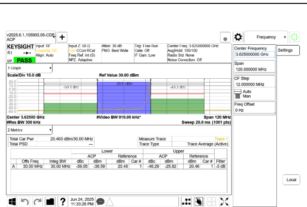
5G NR n48 30MHz QPSK Mid Channel RB1-77 Port A
