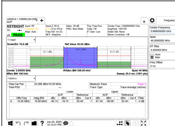
5G NR n48 10MHz QPSK High Channel RB1-0 Port A+B
