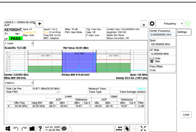
5G NR n48 30MHz QPSK Mid Channel RB1-77 Port B
