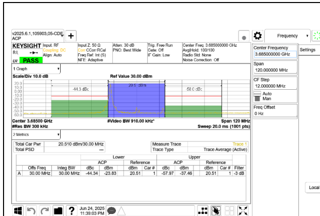
5G NR n48 30MHz QPSK High Channel RB1-0 Port A
