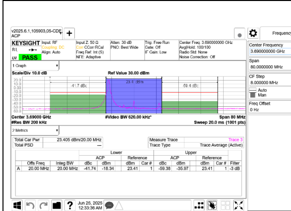
5G NR n48 20MHz QPSK High Channel RB1-0 Port A+B
