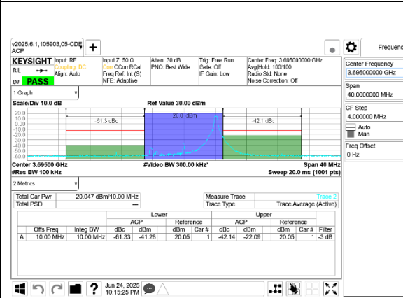
5G NR n48 10MHz QPSK High Channel RB1-23 Port B
