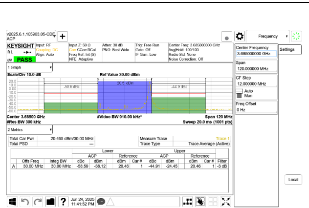
5G NR n48 30MHz QPSK High Channel RB1-77 Port A
