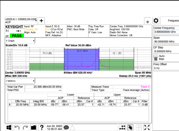
5G NR n48 20MHz QPSK High Channel RB1-50 Port A+B
