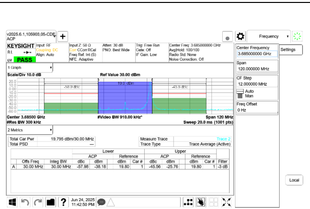
5G NR n48 30MHz QPSK High Channel RB1-77 Port B
