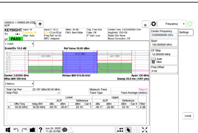
5G NR n48 30MHz QPSK Mid Channel RB1-77 Port A+B
