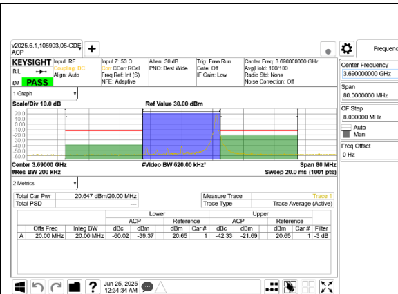
5G NR n48 20MHz QPSK High Channel RB1-50 Port A
