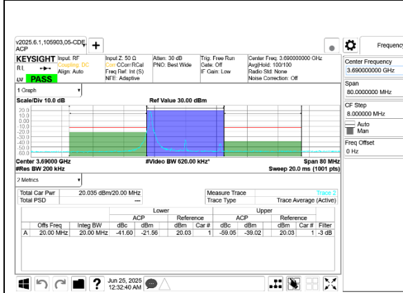
5G NR n48 20MHz QPSK High Channel RB1-0 Port B
