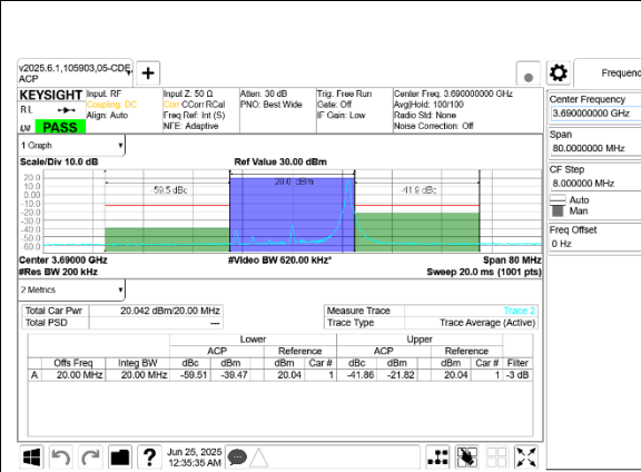
5G NR n48 20MHz QPSK High Channel RB1-50 Port B
