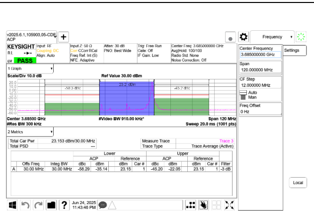
5G NR n48 30MHz QPSK High Channel RB1-77 Port A+B
