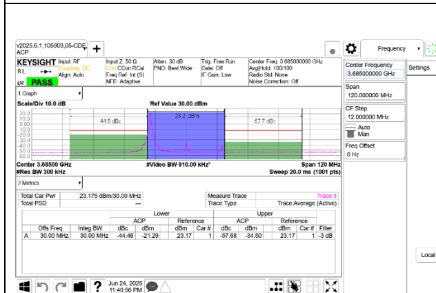
5G NR n48 30MHz QPSK High Channel RB1-0 Port A+B
