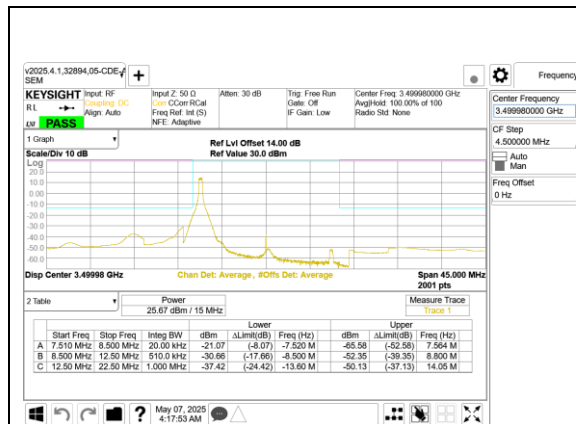
5G NR n77 15MHz BPSK Mid Channel RB1-0 Port A
