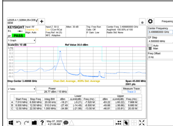
5G NR n77 15MHz BPSK Mid Channel RB1-0 Port A+B
