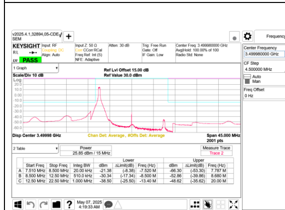
5G NR n77 15MHz BPSK Mid Channel RB1-0 Port B
