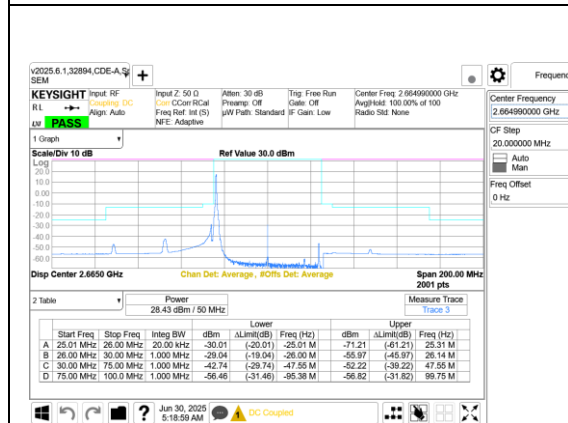
5G NR n41 50MHz BPSK High Channel RB1-0 Port A+B
