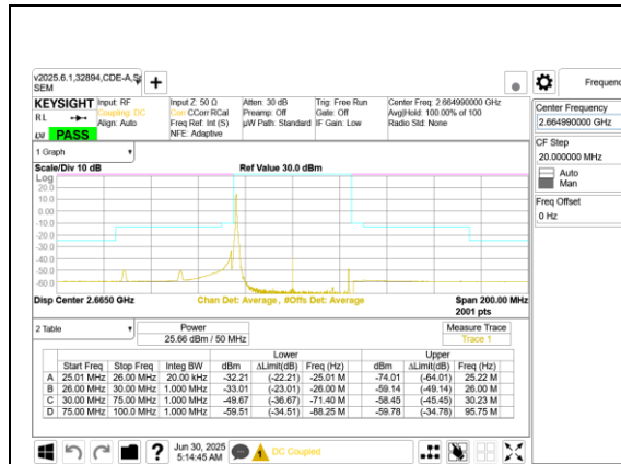
5G NR n41 50MHz BPSK High Channel RB1-0 Port A
