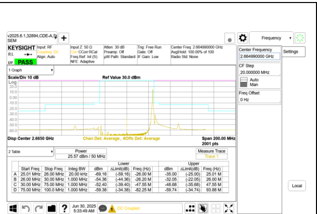
5G NR n41 50MHz BPSK High Channel RB1-132 Port A
