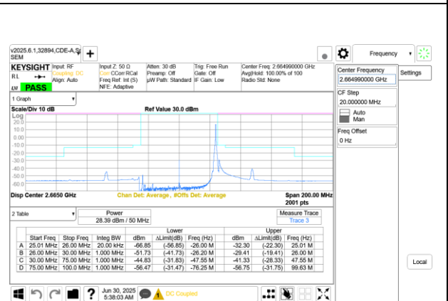
5G NR n41 50MHz BPSK High Channel RB1-132 Port A+B
