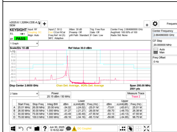
5G NR n41 50MHz BPSK High Channel RB1-0 Port B
