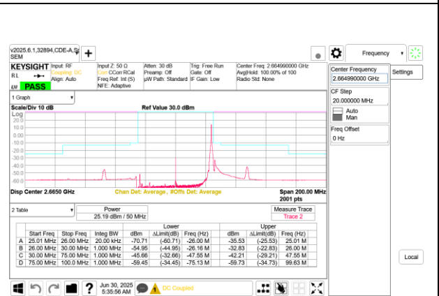
5G NR n41 50MHz BPSK High Channel RB1-132 Port B
