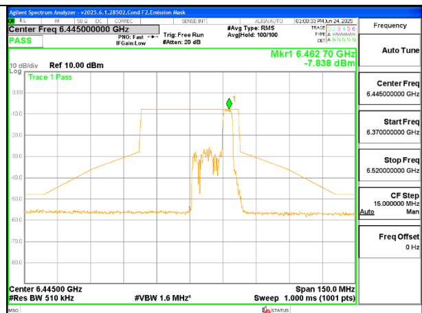
LOW CHANNEL ANT 5 6445
