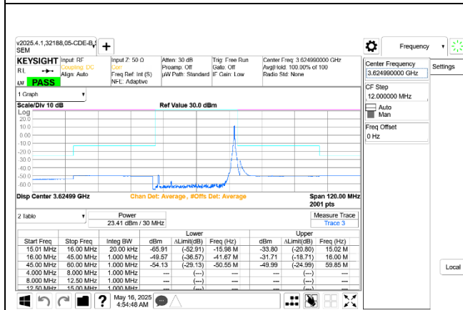
5G NR n48 30MHz QPSK Middle Channel RB1-77 Ant 9+8
