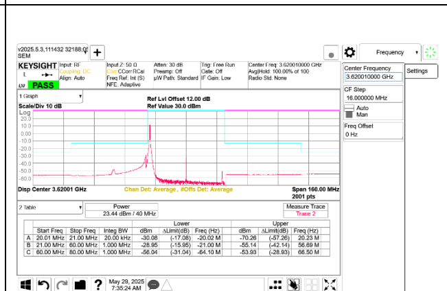
5G NR n48 40MHz QPSK Middle Channel RB1-0 Ant 8
