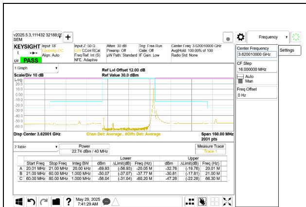
5G NR n48 40MHz QPSK Mid Channel RB1-105 Ant 9
