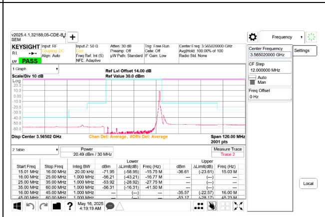
5G NR n48 30MHz QPSK Low Channel RB1-77 Ant 8
