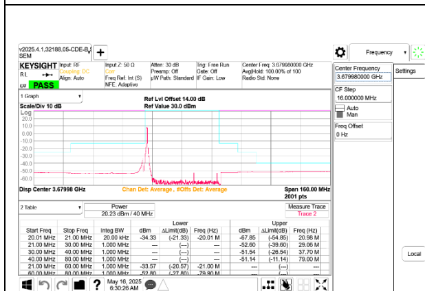
5G NR n48 40MHz QPSK High Channel RB1-0 Ant 8
