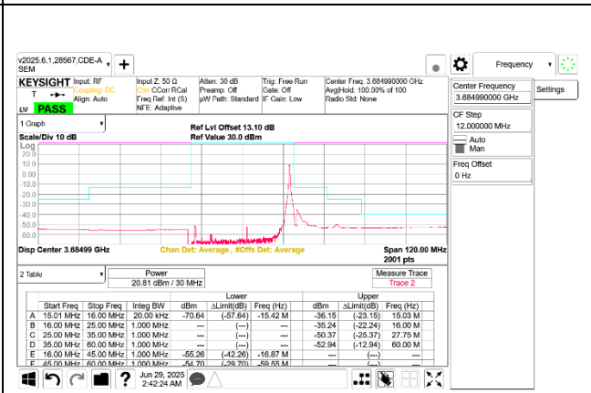
5G NR n48 30MHz QPSK High Channel RB1-77 Ant 8
