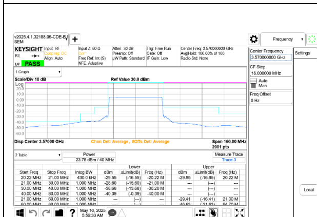
5G NR n48 40MHz QPSK Low Channel RB106-0 Ant 9+8
