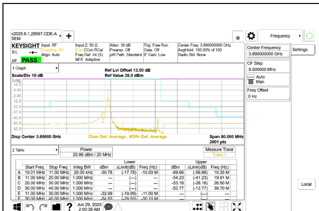
5G NR n48 20MHz QPSK High Channel RB1-0 Ant 9
