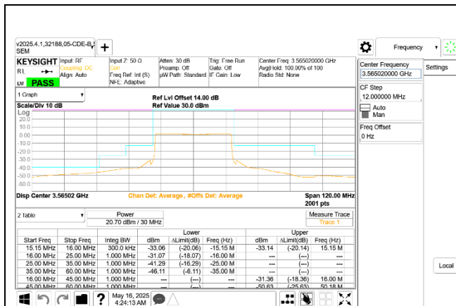
5G NR n48 30MHz QPSK Low Channel RB78-0 Ant 9
