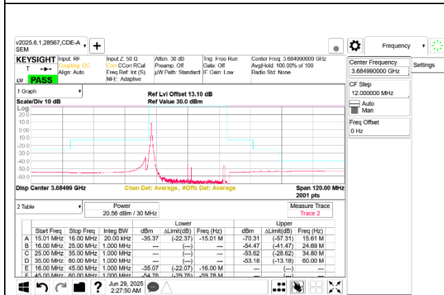
5G NR n48 30MHz QPSK High Channel RB1-0 Ant 8
