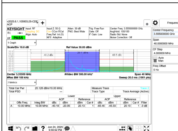
5G NR n48 10MHz QPSK Low Channel RB1-0 Port B
