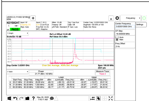
5G NR n48 40MHz QPSK Mid Channel RB1-105 Ant 8
