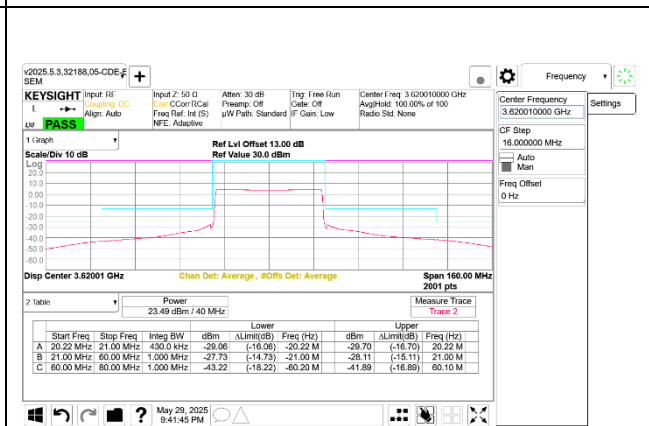
5G NR n48 40MHz QPSK Mid Channel RB106-0 Ant 8
