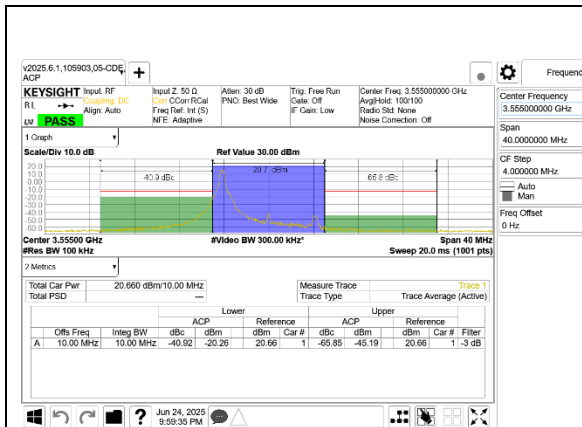
5G NR n48 10MHz QPSK Low Channel RB1-0 Port A
