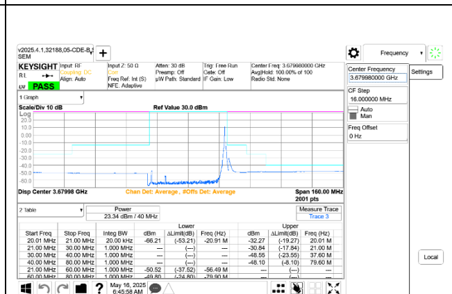
5G NR n48 40MHz QPSK High Channel RB1-105 Ant 9+8
