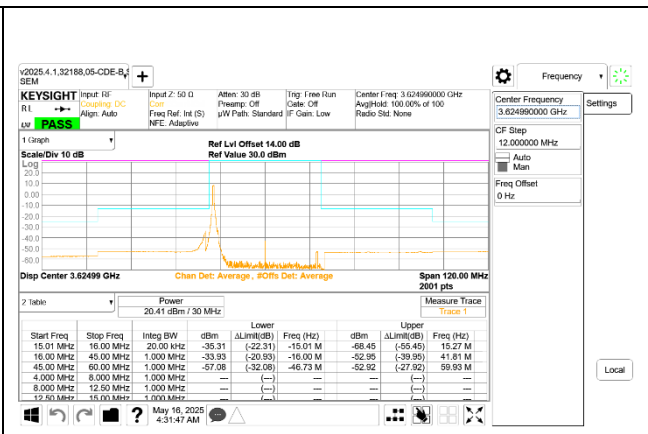
5G NR n48 30MHz QPSK Middle Channel RB1-0 Ant 9
