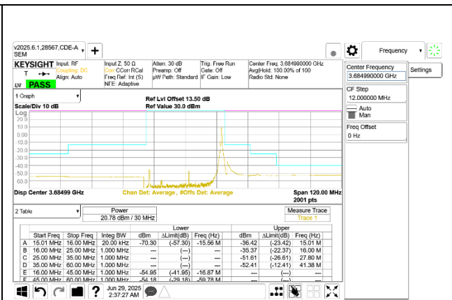
5G NR n48 30MHz QPSK High Channel RB1-77 Ant 9
