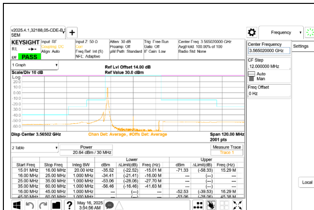
5G NR n48 30MHz QPSK Low Channel RB1-0 Ant 9
