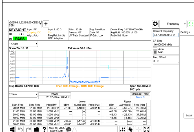
5G NR n48 40MHz QPSK High Channel RB1-0 Ant 9+8
