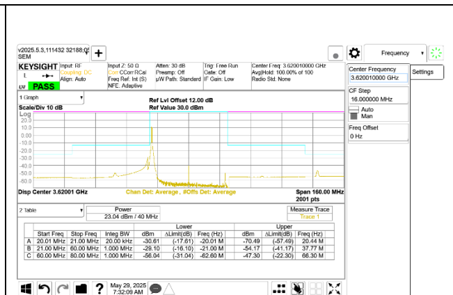
5G NR n48 40MHz QPSK Middle Channel RB1-0 Ant 9
