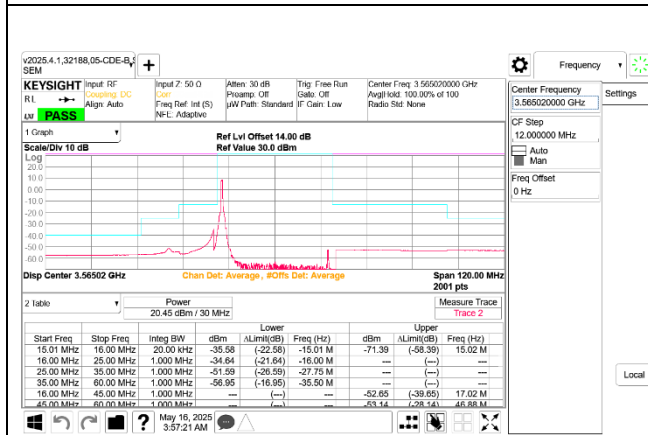
5G NR n48 30MHz QPSK Low Channel RB1-0 Ant 8
