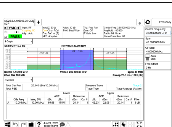
5G NR n48 10MHz QPSK Low Channel RB1-23 Port B
