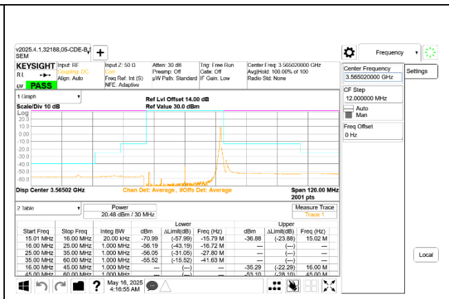
5G NR n48 30MHz QPSK Low Channel RB1-77 Ant 9
