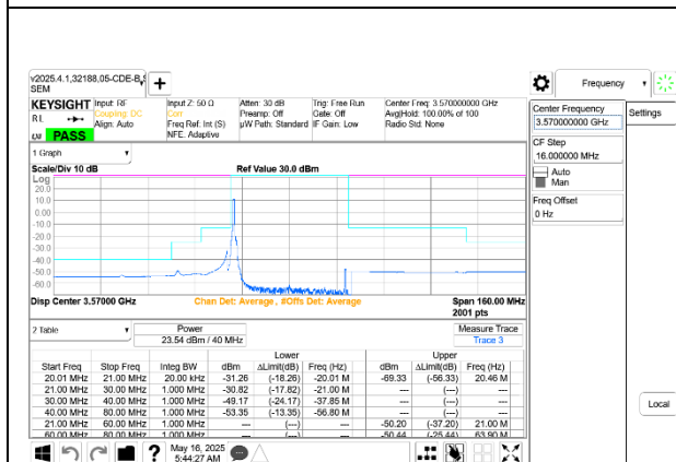
5G NR n48 40MHz QPSK Low Channel RB1-0 Ant 9+8
