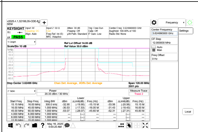
5G NR n48 30MHz QPSK Middle Channel RB78-0 Ant 8
