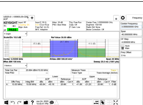
5G NR n48 10MHz QPSK Low Channel RB1-23 Port A, ID: 27957
