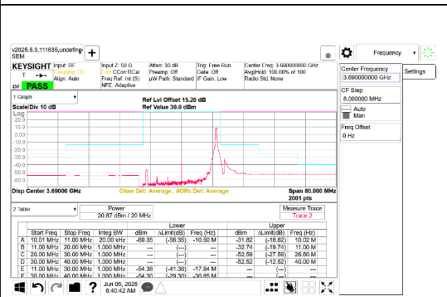
5G NR n48 20MHz QPSK High Channel RB1-50 Ant 8
