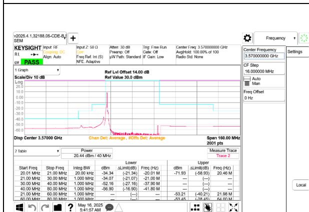
5G NR n48 40MHz QPSK Low Channel RB1-0 Ant 8
