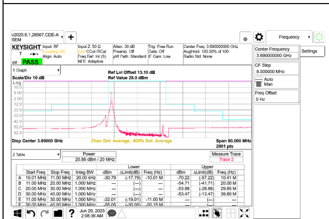
5G NR n48 20MHz QPSK High Channel RB1-0 Ant 8
