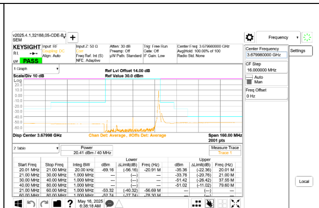
5G NR n48 40MHz QPSK High Channel RB1-105 Ant 9
