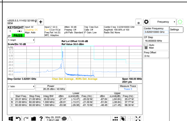
5G NR n48 40MHz QPSK Middle Channel RB1-0 Ant 9+8
