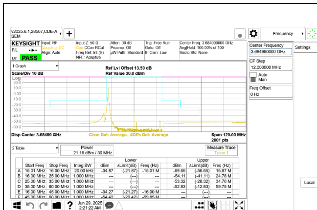
5G NR n48 30MHz QPSK High Channel RB1-0 Ant 9
