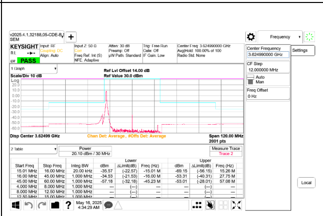
5G NR n48 30MHz QPSK Middle Channel RB1-0 Ant 8
