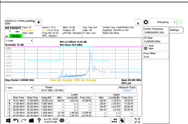
5G NR n48 20MHz QPSK High Channel RB1-50 Ant 9+8
