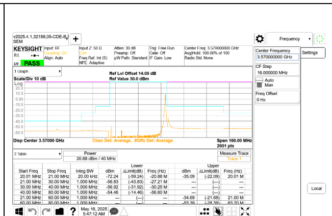
5G NR n48 40MHz QPSK Low Channel RB1-105 Ant 9
