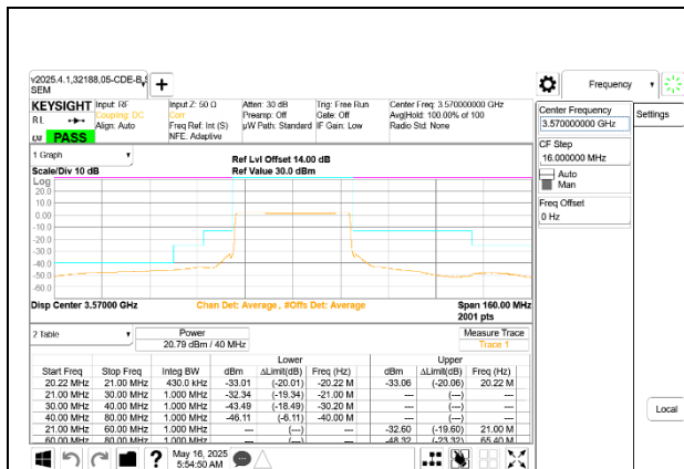
5G NR n48 40MHz QPSK Low Channel RB106-0 Ant 9
