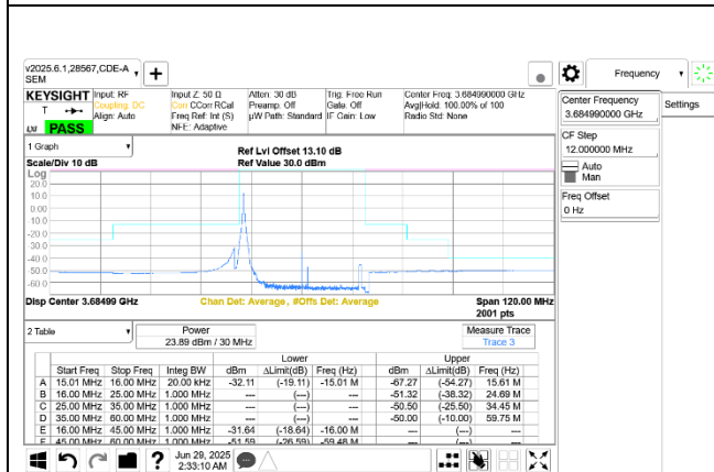
5G NR n48 30MHz QPSK High Channel RB1-0 Ant 9+8
