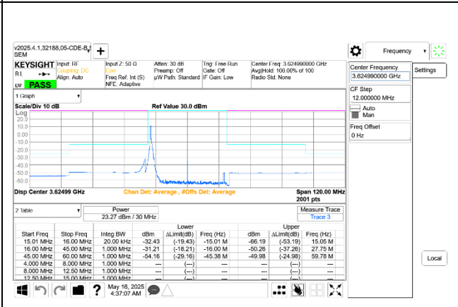
5G NR n48 30MHz QPSK Middle Channel RB1-0 Ant 9+8
