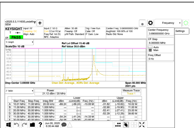
5G NR n48 20MHz QPSK High Channel RB1-50 Ant 9
