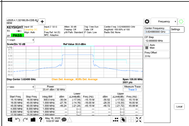
5G NR n48 30MHz QPSK Middle Channel RB78-0 Ant 9+8
