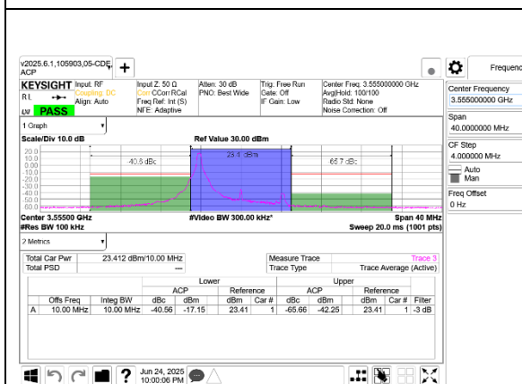
5G NR n48 10MHz QPSK Low Channel RB1-0 Port A+B
