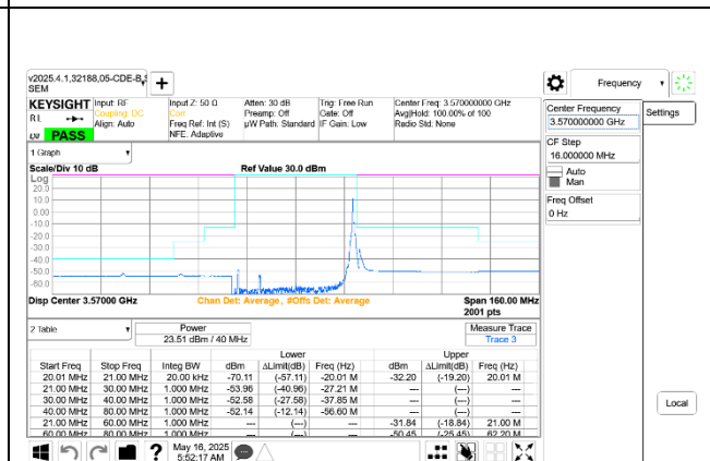
5G NR n48 40MHz QPSK Low Channel RB1-105 Ant 9+8
