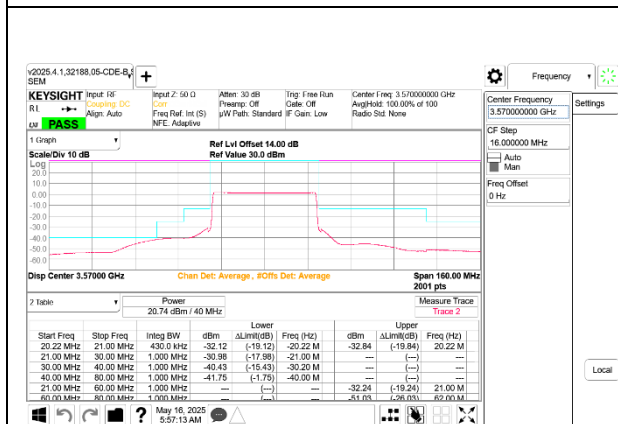
5G NR n48 40MHz QPSK Low Channel RB106-0 Ant 8
