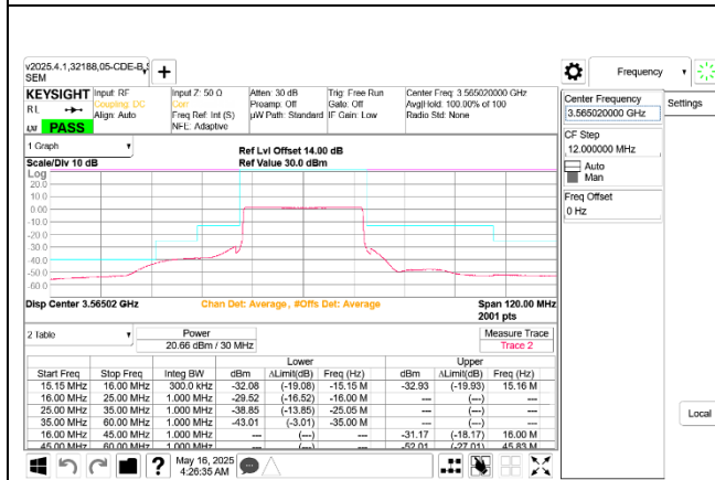
5G NR n48 30MHz QPSK Low Channel RB78-0 Ant 8
