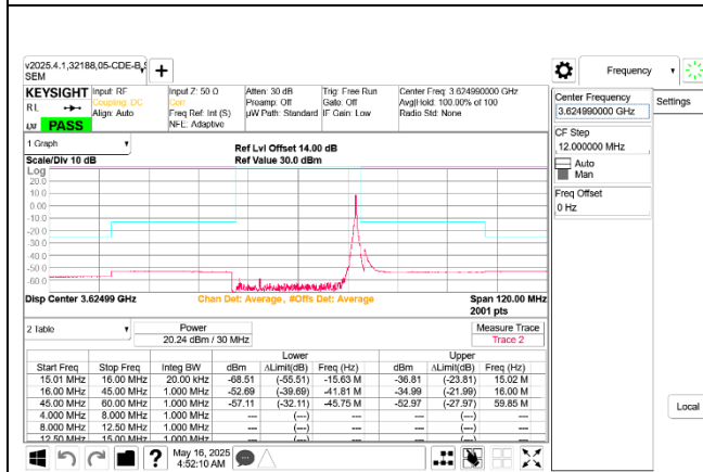
5G NR n48 30MHz QPSK Middle Channel RB1-77 Ant 8
