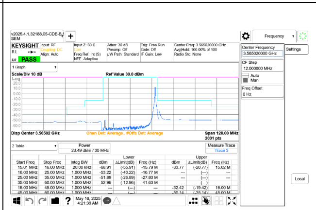
5G NR n48 30MHz QPSK Low Channel RB1-77 Ant 9+8
