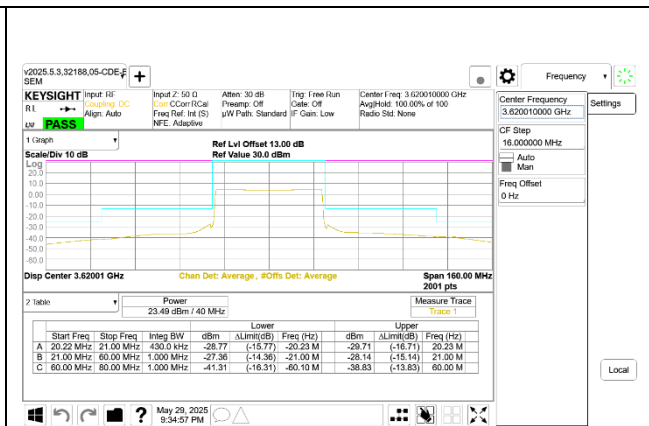
5G NR n48 40MHz QPSK Mid Channel RB106-0 Ant 9
