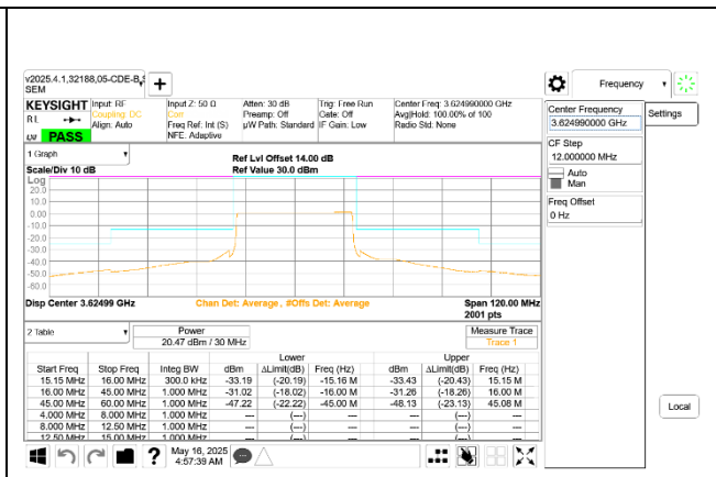
5G NR n48 30MHz QPSK Middle Channel RB78-0 Ant 9
