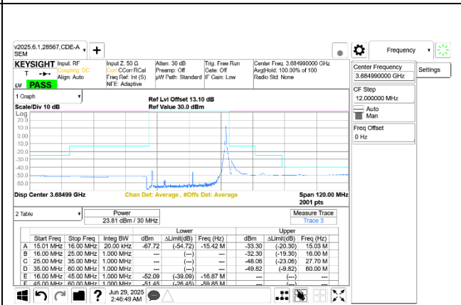
5G NR n48 30MHz QPSK High Channel RB1-77 Ant 9+8
