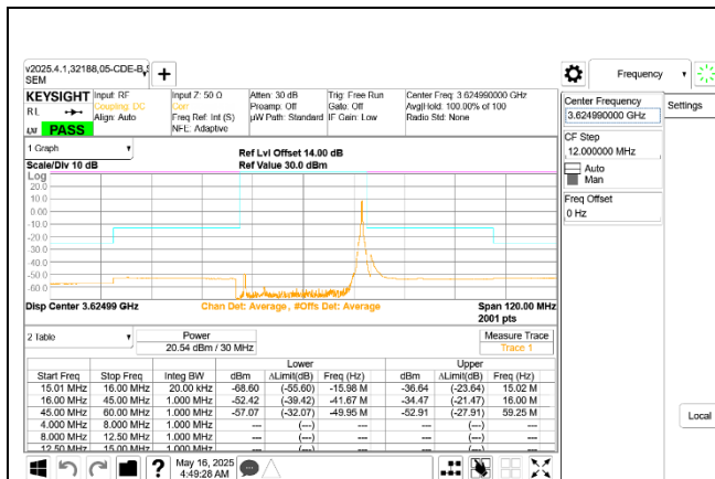
5G NR n48 30MHz QPSK Middle Channel RB1-77 Ant 9
