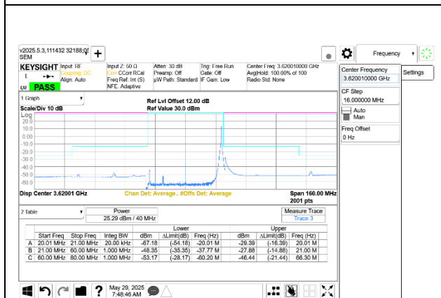
5G NR n48 40MHz QPSK Mid Channel RB1-105 Ant 9+8
