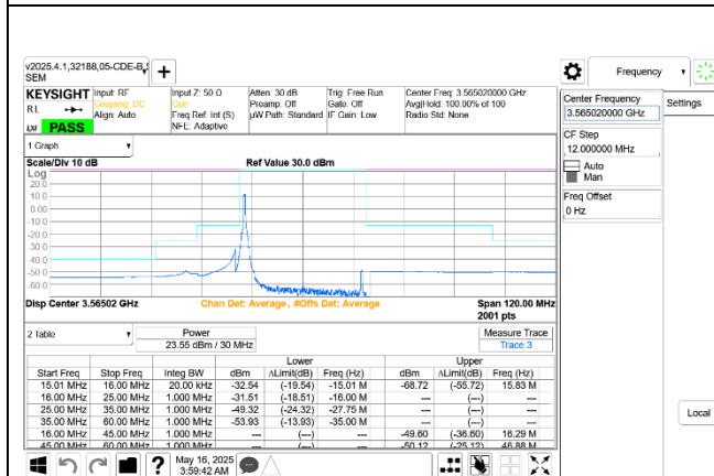
5G NR n48 30MHz QPSK Low Channel RB1-0 Ant 9+8
