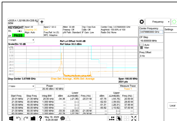
5G NR n48 40MHz QPSK High Channel RB1-0 Ant 9
