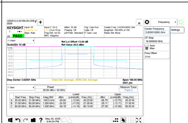
5G NR n48 40MHz QPSK Mid Channel RB106-0 Ant 9+8
