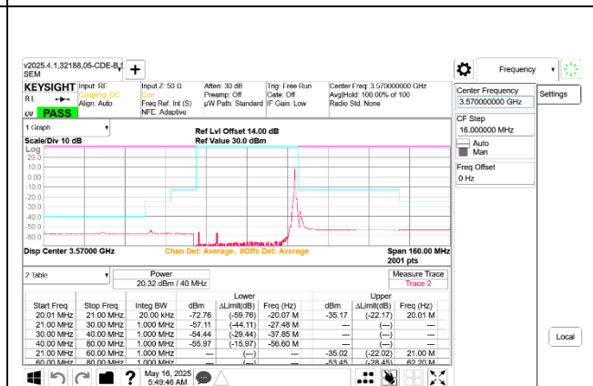
5G NR n48 40MHz QPSK Low Channel RB1-105 Ant 8
