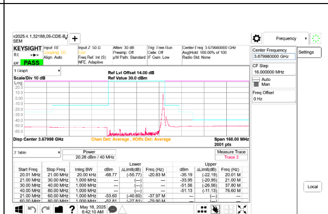
5G NR n48 40MHz QPSK High Channel RB1-105 Ant 8
