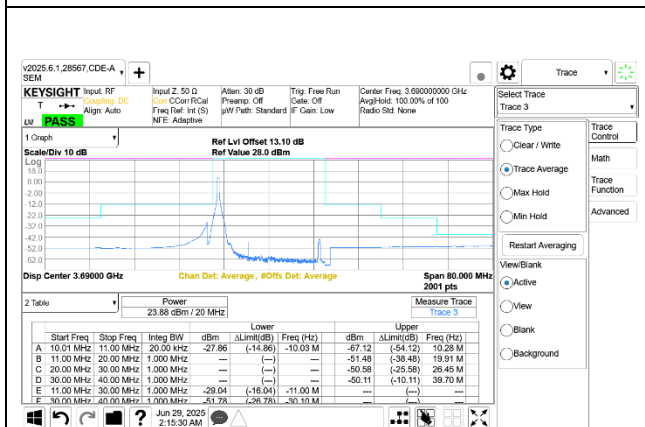
5G NR n48 20MHz QPSK High Channel RB1-0 Ant 9+8
