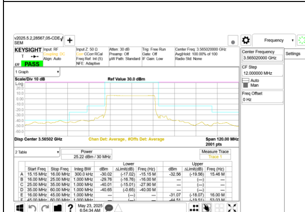
5G NR n48 30MHz BPSK Low Channel RB75-0
