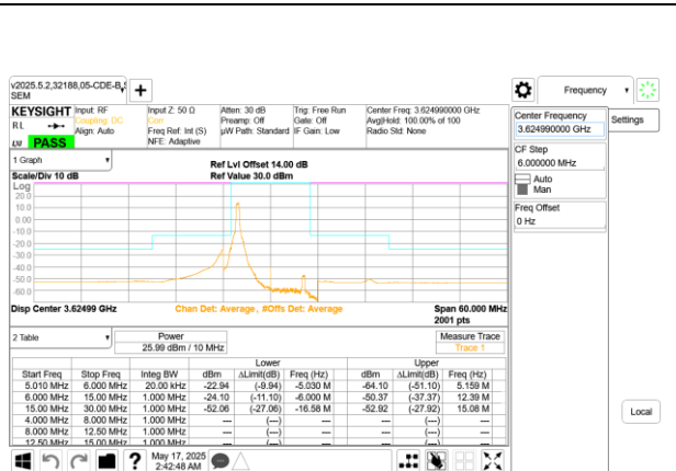
5G NR n48 10MHz BPSK Middle Channel RB1-0
