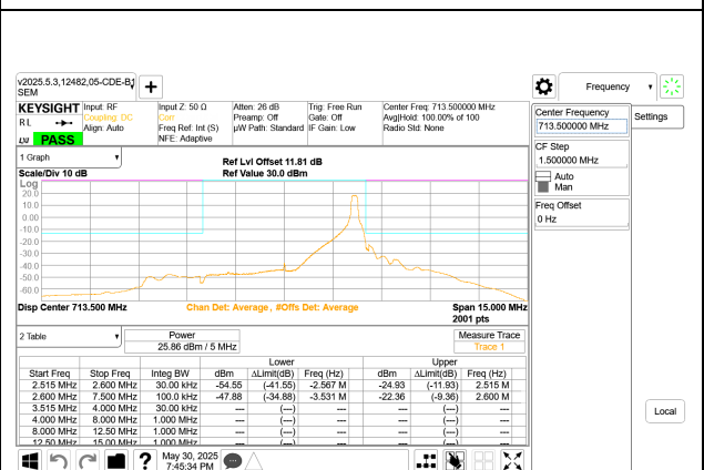
LTE B17 5MHz QPSK High Channel RB1-24
