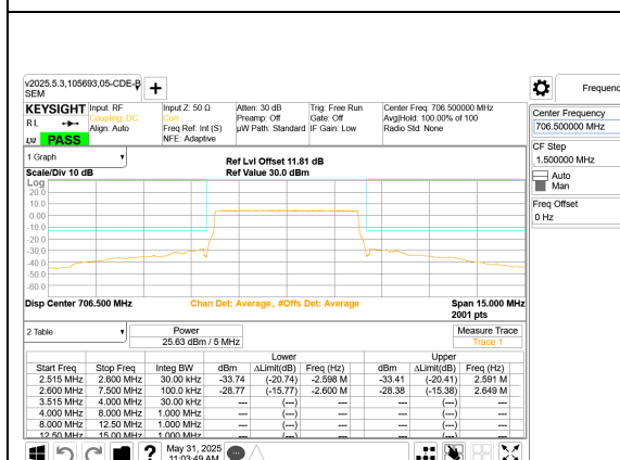
LTE B17 5MHz QPSK Low Channel RB25-0
