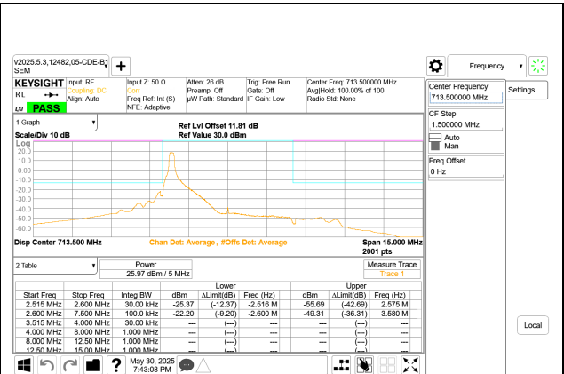
LTE B17 5MHz QPSK High Channel RB1-0
