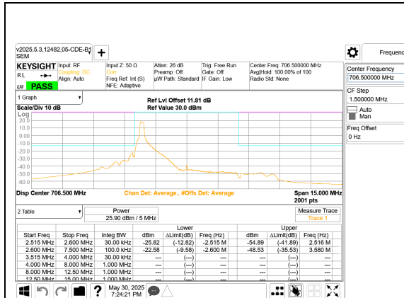
LTE B17 5MHz QPSK Low Channel RB1-0
