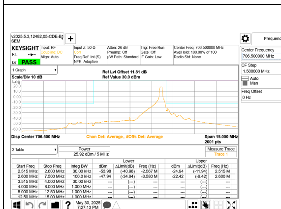
LTE B17 5MHz QPSK Low Channel RB1-24
