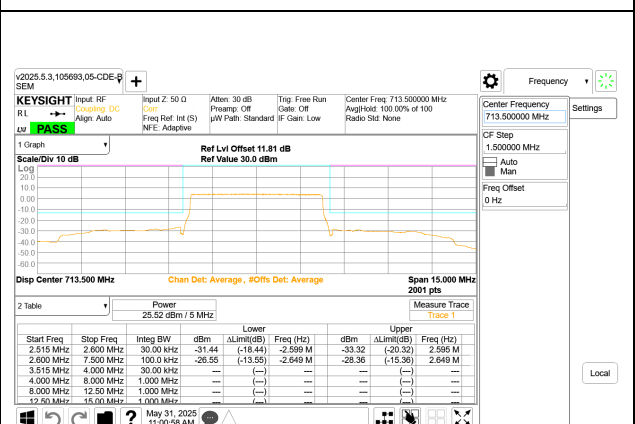
LTE B17 5MHz QPSK High Channel RB25-0
