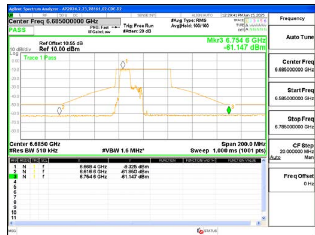
MID CHANNEL 6685
