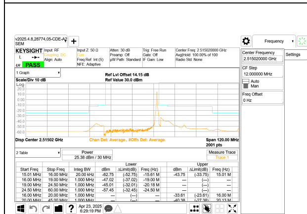
5G NR n41 30MHz BPSK Low Channel RB1-77
