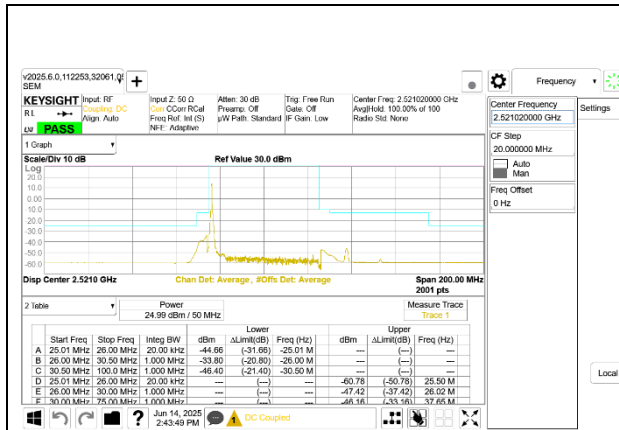
5G NR n41 50MHz BPSK Low Channel RB1-0
