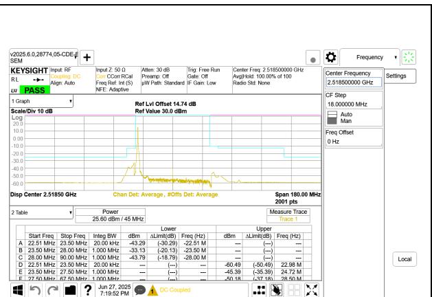
5G NR n41 45MHz BPSK Low Channel RB1-0
