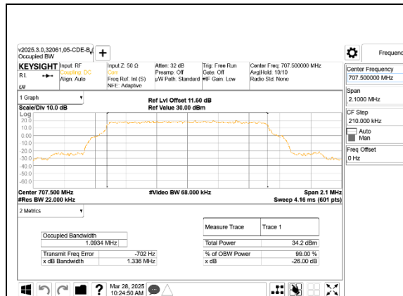
LTE B12 1.4MHz QPSK Middle Channel RB6-0
