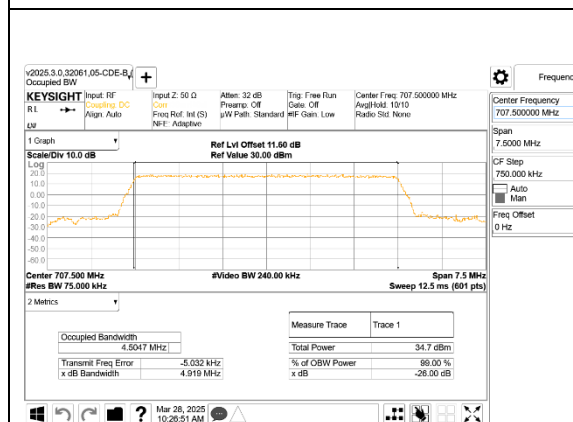
LTE B12 5MHz QPSK Middle Channel RB25-0
