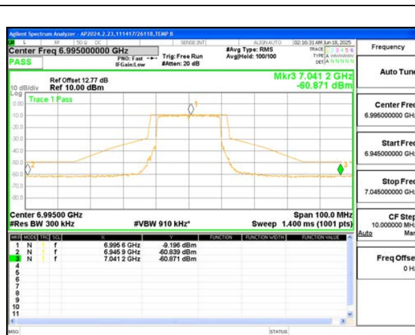
MID CHANNEL ANT 6 6995
