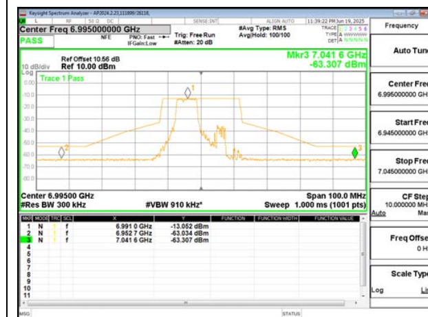
MID CHANNEL ANT 6 6995
