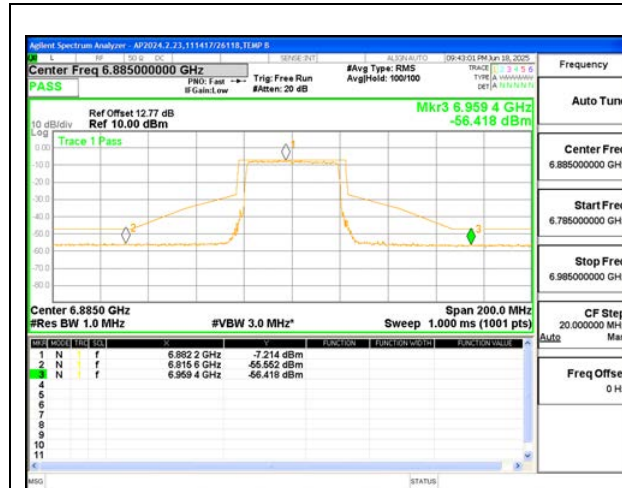
STRADDLE CHANNEL, ANT 5 6885
