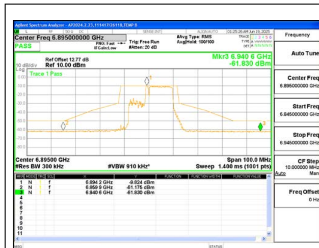
LOW CHANNEL ANT 6 6895
