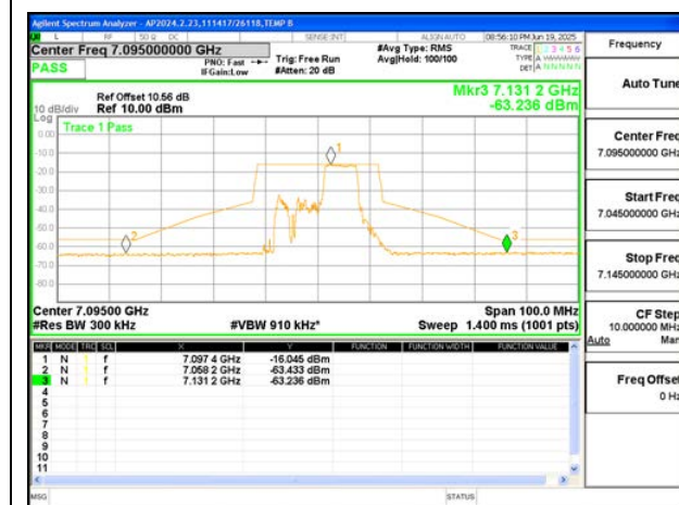
HIGH CHANNEL ANT 6 7095
