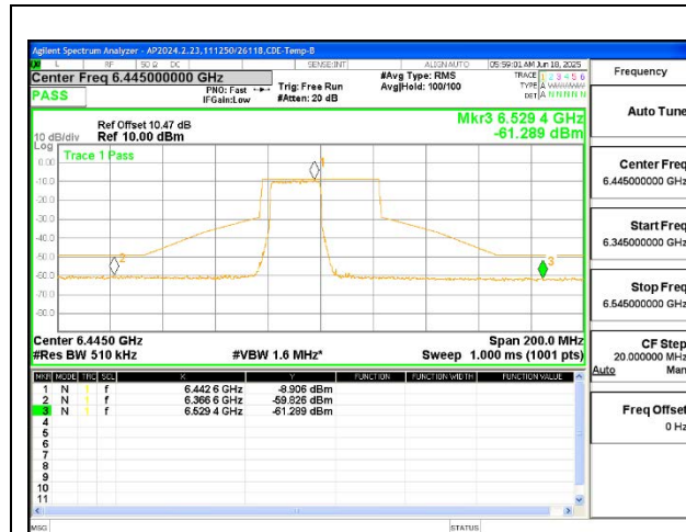
LOW CHANNEL ANT 6 6445
