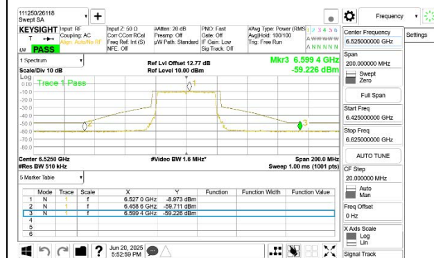
STRADDLE CHANNEL ANT 5 6525
