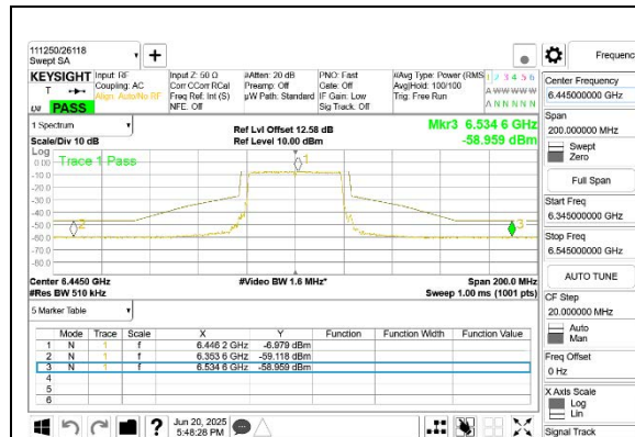
LOW CHANNEL ANT 5 6445
