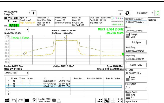
MID CHANNEL ANT 5 6485
