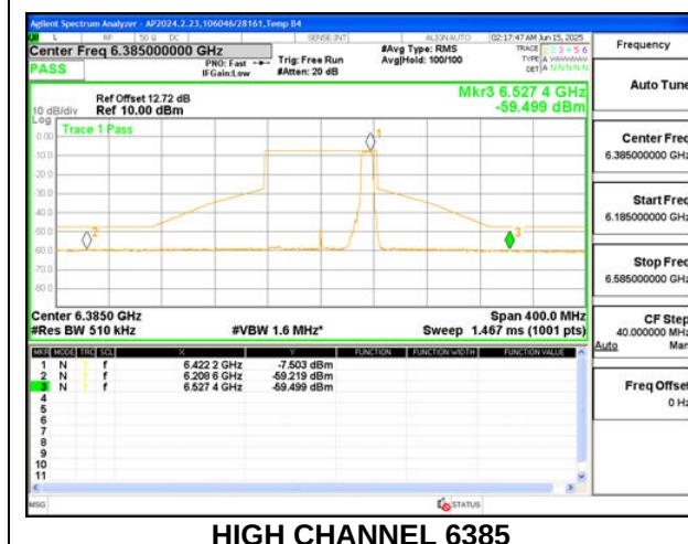
HIGH CHANNEL 6385
