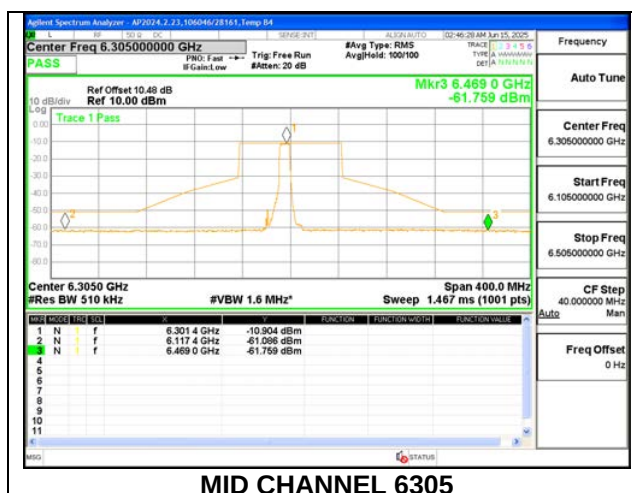
MID CHANNEL 6305
