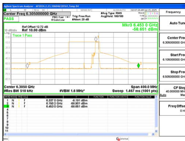
MID CHANNEL 6305
