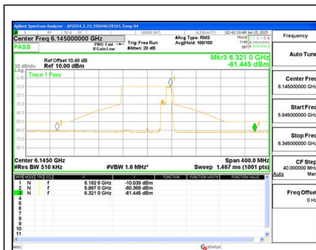
LOW CHANNEL 6145
