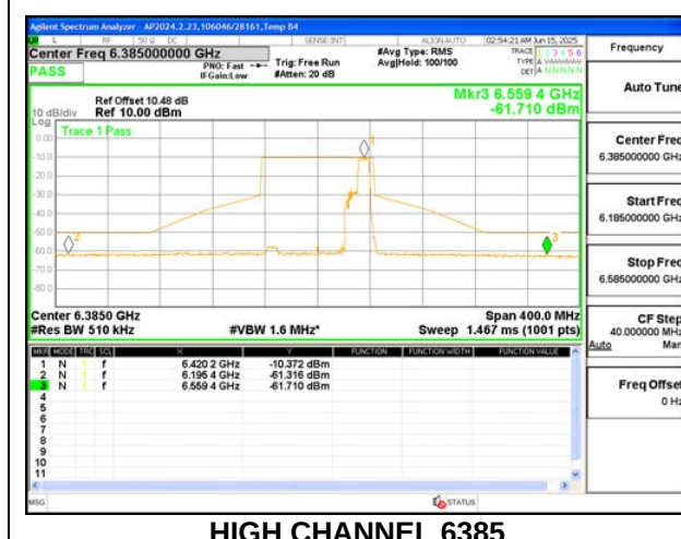
HIGH CHANNEL 6385
