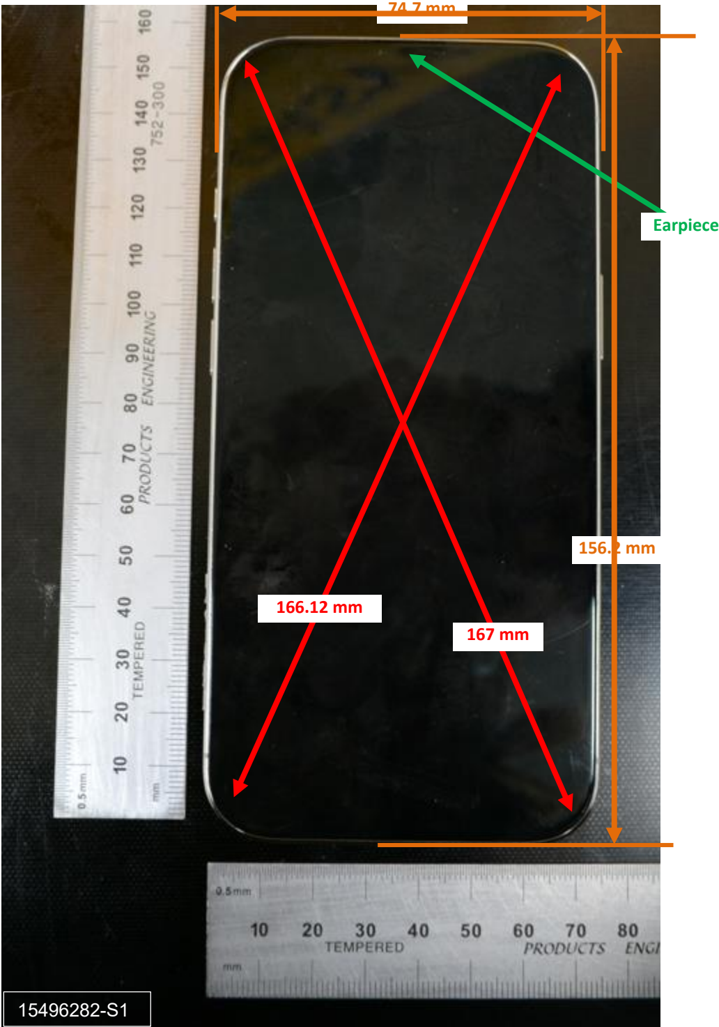
Photograph 1: Overall Dimensions
