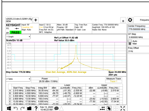
LTE B13 5MHz QPSK Low Channel RB1-24
