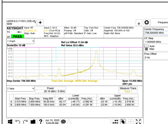
LTE B17 5MHz QPSK Low Channel RB1-24
