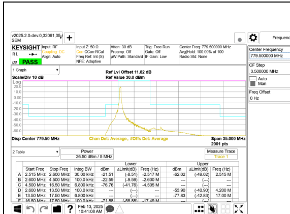
LTE B13 5MHz QPSK Low Channel RB1-0
