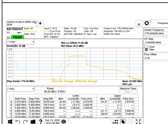
LTE B13 5MHz QPSK Low Channel RB25-0
