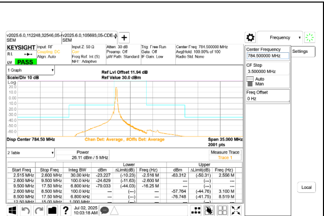
LTE B13 5MHz QPSK High Channel RB1-0
