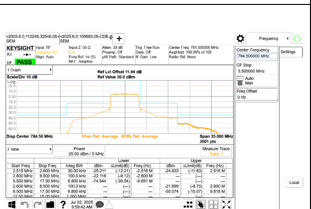
LTE B13 5MHz QPSK High Channel RB25-0
