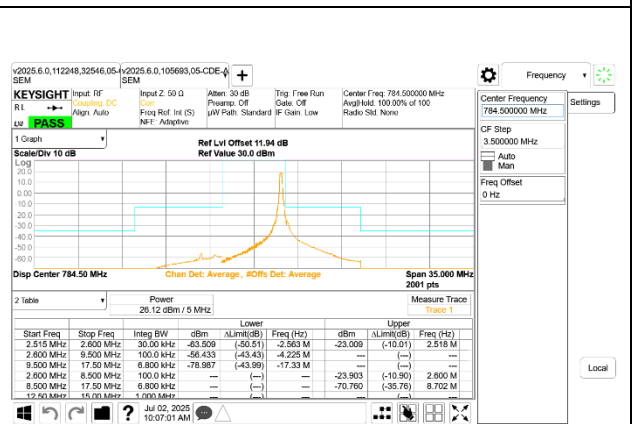
LTE B13 5MHz QPSK High Channel RB1-24
