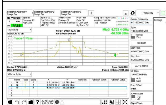
MID CHANNEL ANT 6 6715
