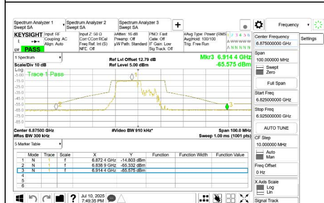
STRADDLE CHANNEL ANT 6 6875
