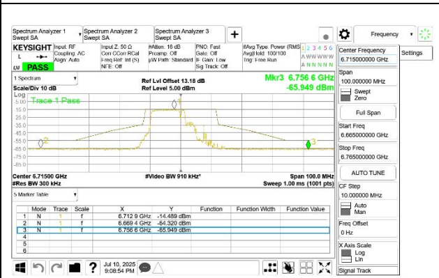
MID CHANNEL ANT 5 6715
