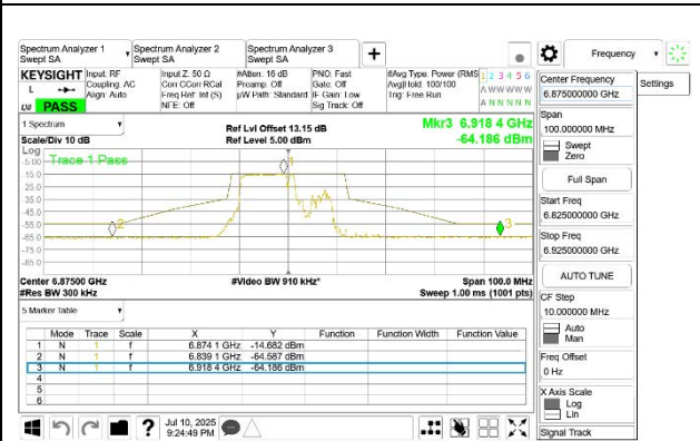
STRADDLE CHANNEL ANT 5 6875
