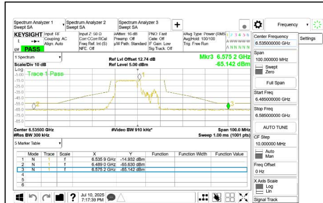
LOW CHANNEL ANT 6 6535
