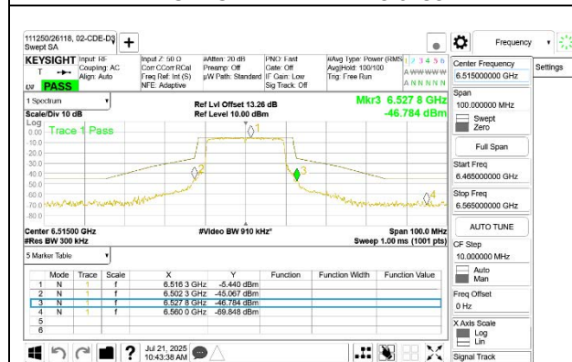
HIGH CHANNEL ANT 5 6515
