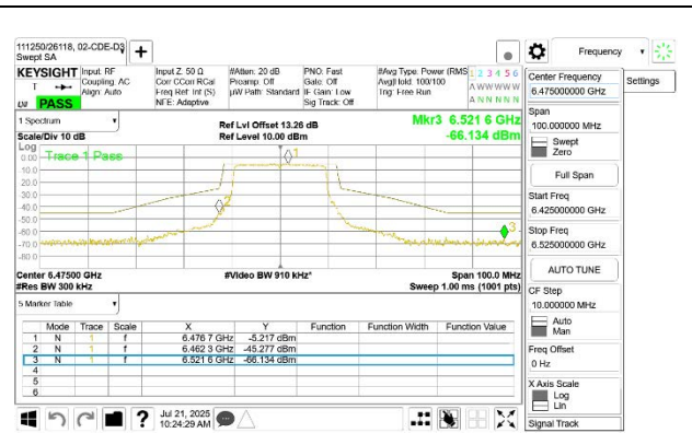
MID CHANNEL ANT 5 6475
