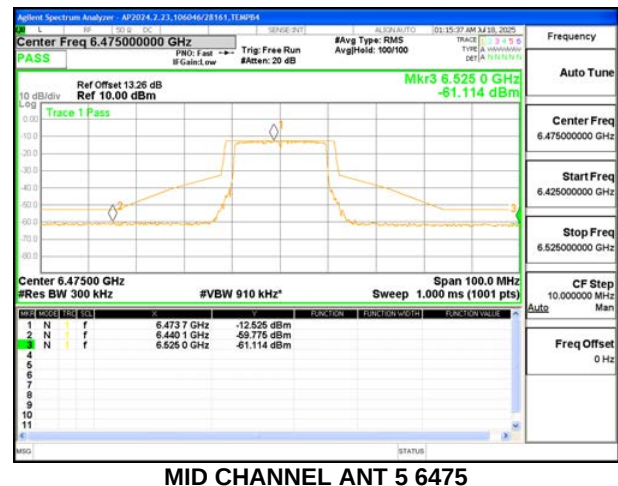
MID CHANNEL ANT 5 6475
