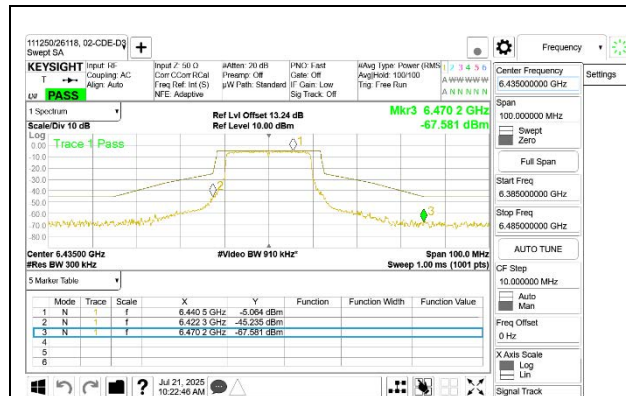
LOW CHANNEL ANT 5 6435
