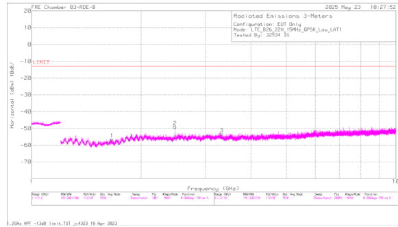
A3258 LTE B26 QPSK Low Channel Horizontal
