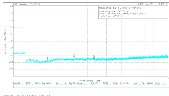
A3258 LTE B26 QPSK Low Channel Vertical
