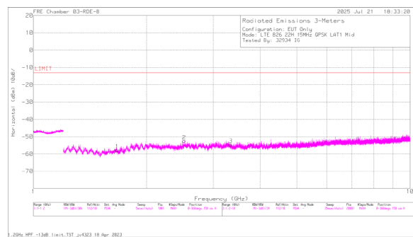
A3521 LTE B26 QPSK Middle Channel Horizontal
