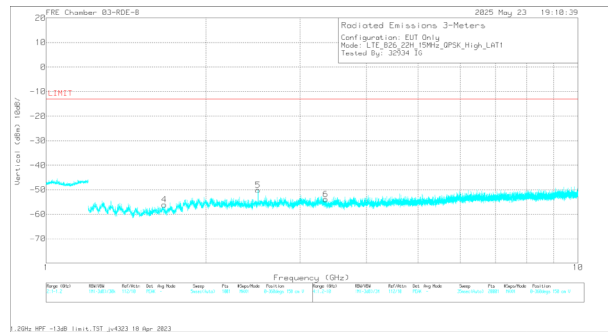
A3258 LTE B26 QPSK High Channel Vertical
