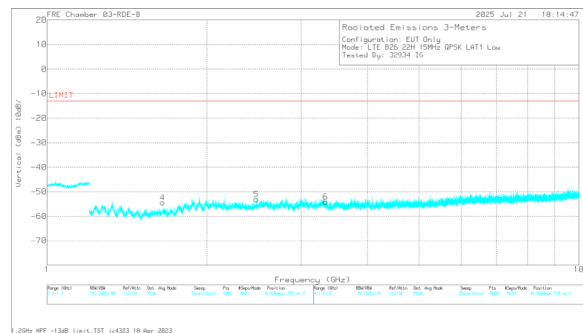
A3521 LTE B26 QPSK Low Channel Vertical
