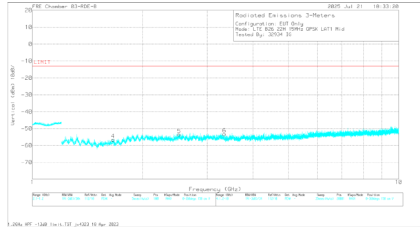
A3519 LTE B26 QPSK Middle Channel Vertical
