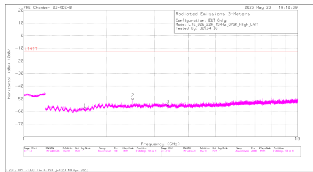
A3258 LTE B26 QPSK High Channel Horizontal
