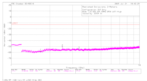
A3521 LTE B26 QPSK High Channel Horizontal
