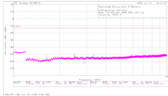
A3521 LTE B26 QPSK Low Channel Horizontal
