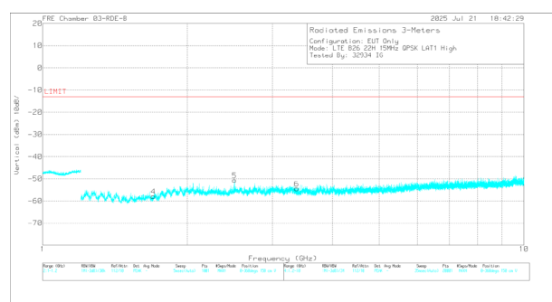
A3521 LTE B26 QPSK High Channel Vertical
