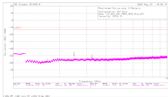
A3258 LTE B26 QPSK Mid Channel Horizontal
