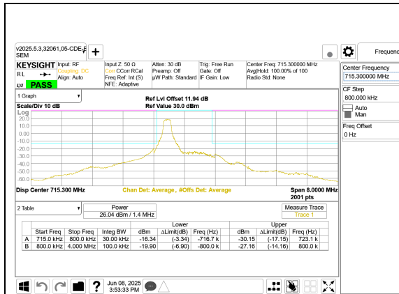
LTE B12 1.4MHz QPSK High Channel RB1-0
