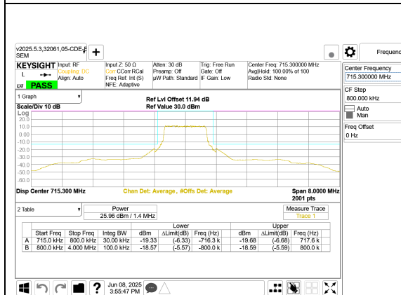
LTE B12 1.4MHz QPSK High Channel RB6-0
