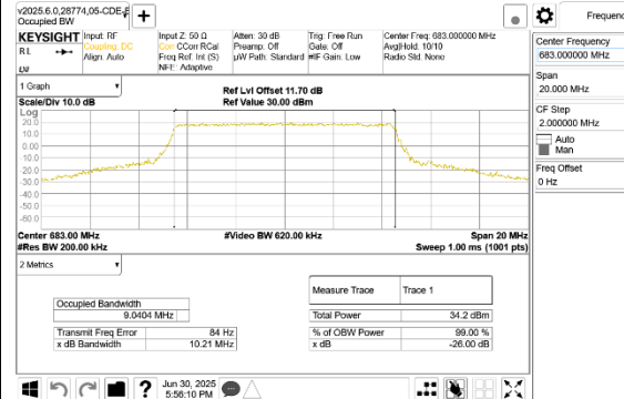
LTE B71 10MHz QPSK Middle Channel RB50-0
