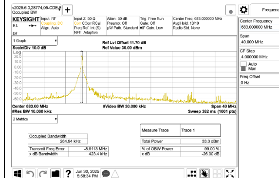
LTE B71 20MHz QPSK Middle Channel RB1-0
