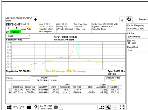
LTE B12 1.4MHz QPSK High Channel RB1-5
