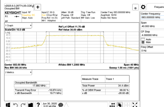
LTE B71 20MHz QPSK Middle Channel RB100-0
