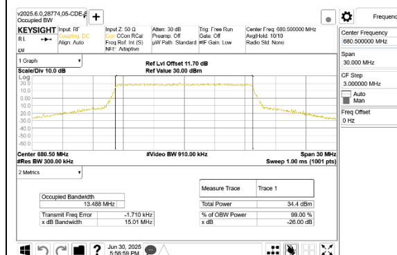
LTE B71 15MHz QPSK Middle Channel RB75-0
