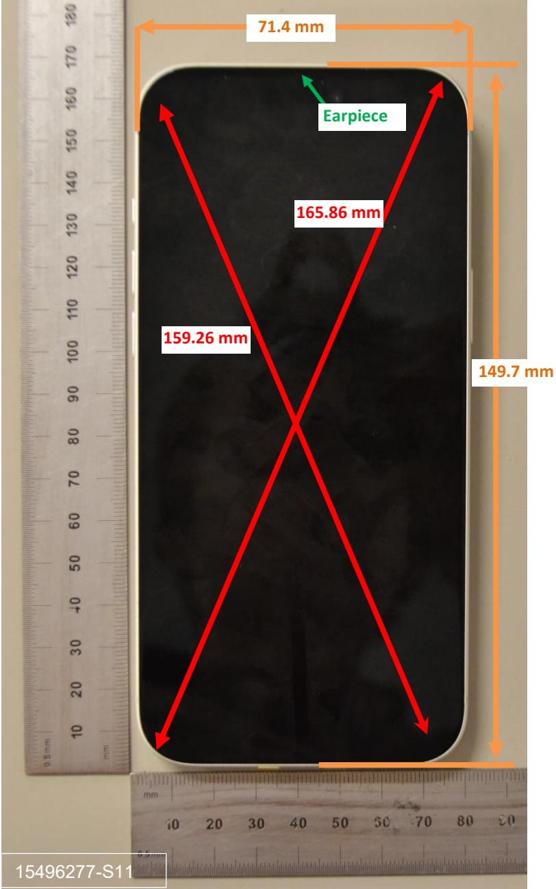
Photograph 1: Overall Dimensions
