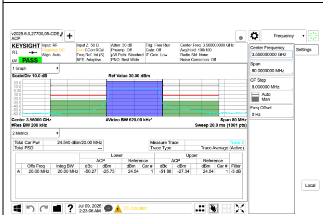
5G NR n48 20MHz BPSK Low Channel RB50-0 Ant 8
