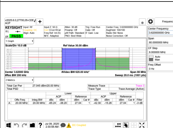
5G NR n48 20MHz BPSK Middle Channel RB1-50 Ant 9+8
