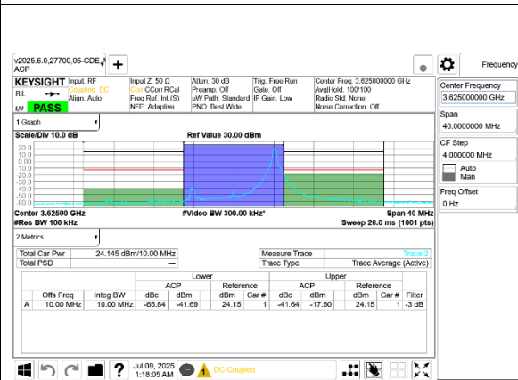
5G NR n48 10MHz BPSK Middle Channel RB1-23 Ant 8
