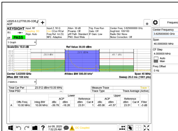
5G NR n48 10MHz BPSK Middle Channel RB1-0 Ant 9
