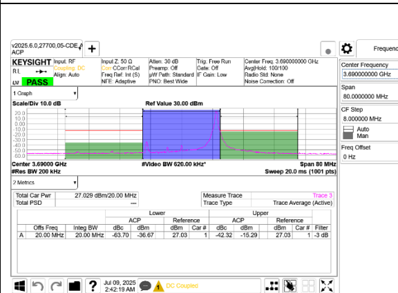
5G NR n48 20MHz BPSK High Channel RB1-50 Ant 9+8
