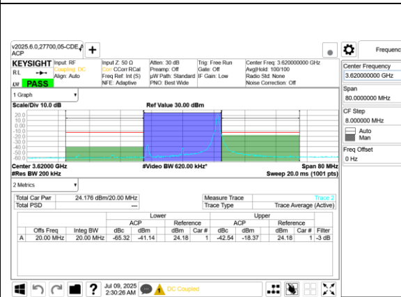
5G NR n48 20MHz BPSK Middle Channel RB1-50 Ant 8
