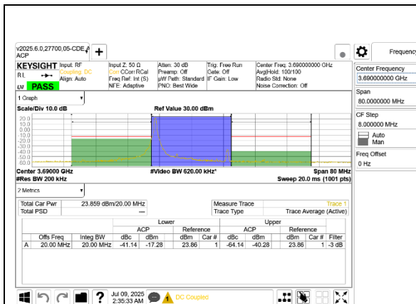
5G NR n48 20MHz BPSK High Channel RB1-0 Ant 9
