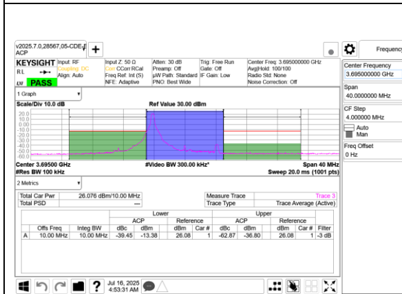
5G NR n48 10MHz BPSK High Channel RB1-0 Ant 9+8
