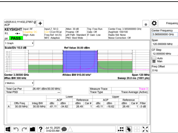
5G NR n48 30MHz BPSK Low Channel RB1-77 Ant 9+8
