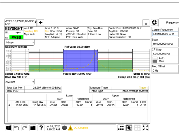
5G NR n48 10MHz BPSK High Channel RB1-23 Ant 9
