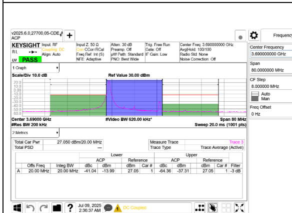
5G NR n48 20MHz BPSK High Channel RB1-0 Ant 9+8
