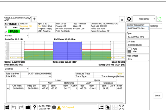
5G NR n48 20MHz BPSK Middle Channel RB50-0 Ant 9
