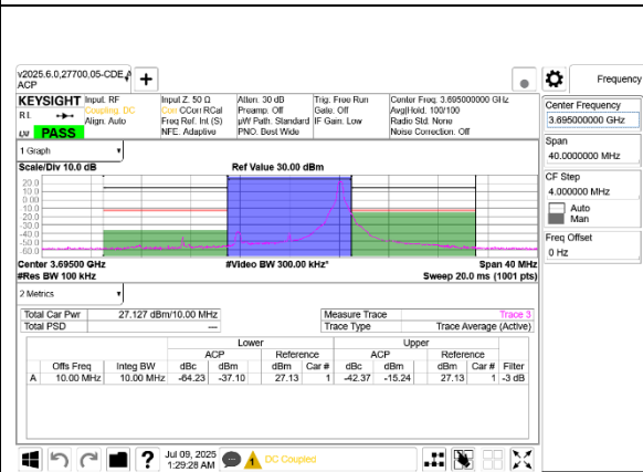
5G NR n48 10MHz BPSK High Channel RB1-23 Ant 9+8
