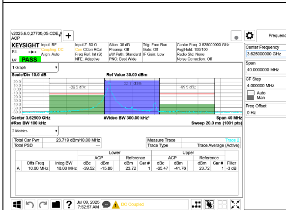
5G NR n48 10MHz BPSK Middle Channel RB1-0 Ant 8
