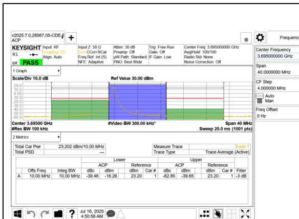
5G NR n48 10MHz BPSK High Channel RB1-0 Ant 9
