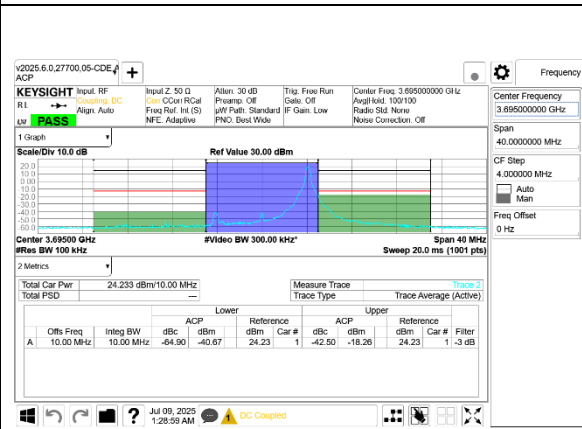
5G NR n48 10MHz BPSK High Channel RB1-23 Ant 8
