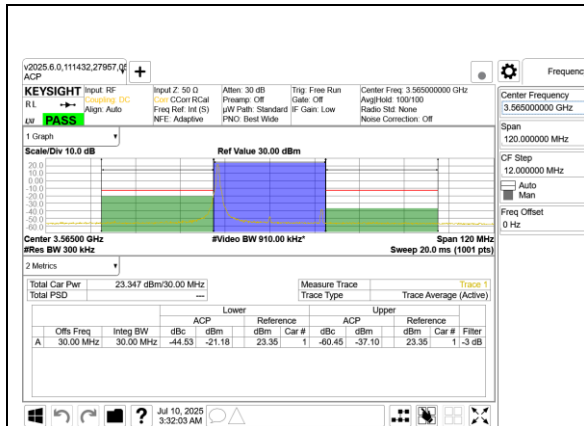
5G NR n48 30MHz BPSK Low Channel RB1-0 Ant 9
