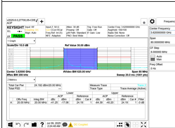
5G NR n48 20MHz BPSK Middle Channel RB1-0 Ant 8
