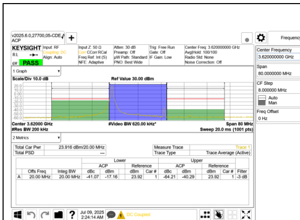
5G NR n48 20MHz BPSK Middle Channel RB1-0 Ant 9
