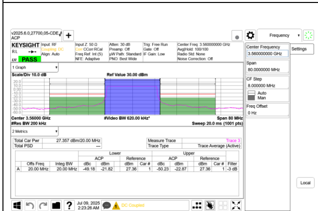
5G NR n48 20MHz BPSK Low Channel RB50-0 Ant 9+8
