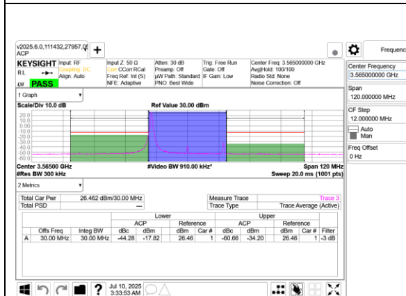
5G NR n48 30MHz BPSK Low Channel RB1-0 Ant 9+8
