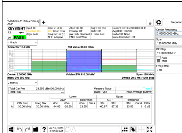
5G NR n48 30MHz BPSK Low Channel RB1-0 Ant 8
