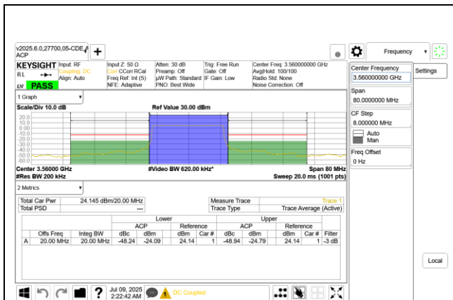
5G NR n48 20MHz BPSK Low Channel RB50-0 Ant 9
