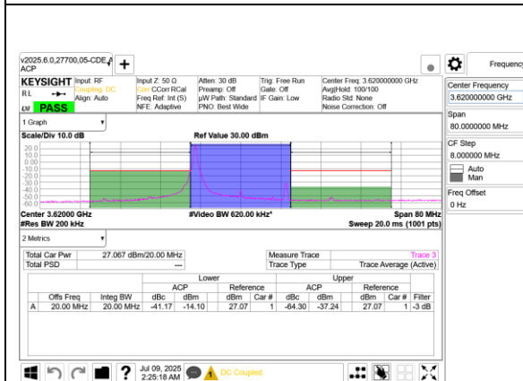
5G NR n48 20MHz BPSK Middle Channel RB1-0 Ant 9+8
