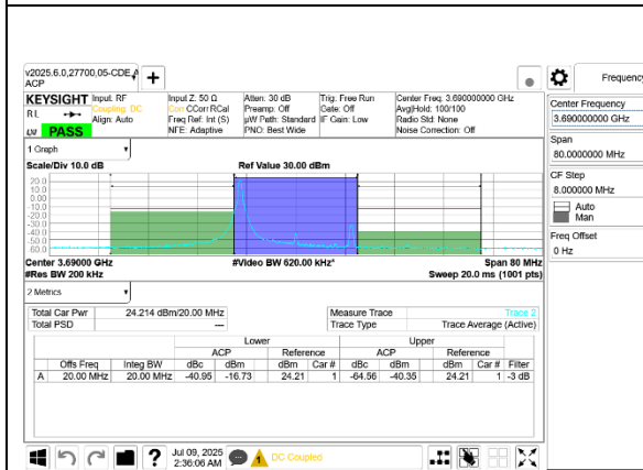
5G NR n48 20MHz BPSK High Channel RB1-0 Ant 8
