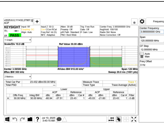
5G NR n48 30MHz BPSK Low Channel RB1-77 Ant 9
