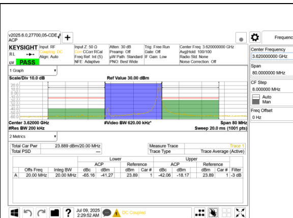
5G NR n48 20MHz BPSK Middle Channel RB1-50 Ant 9
