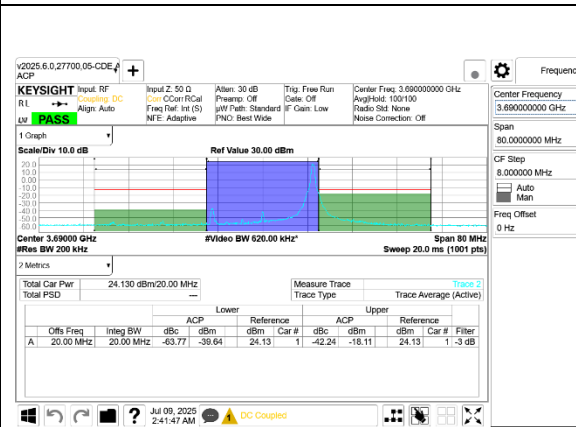
5G NR n48 20MHz BPSK High Channel RB1-50 Ant 8
