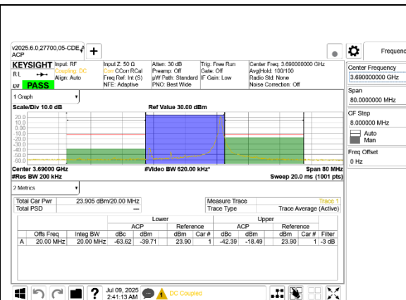
5G NR n48 20MHz BPSK High Channel RB1-50 Ant 9
