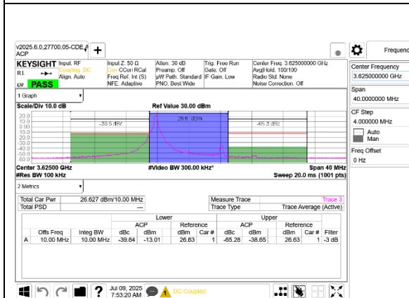
5G NR n48 10MHz BPSK Middle Channel RB1-0 Ant 9+8
