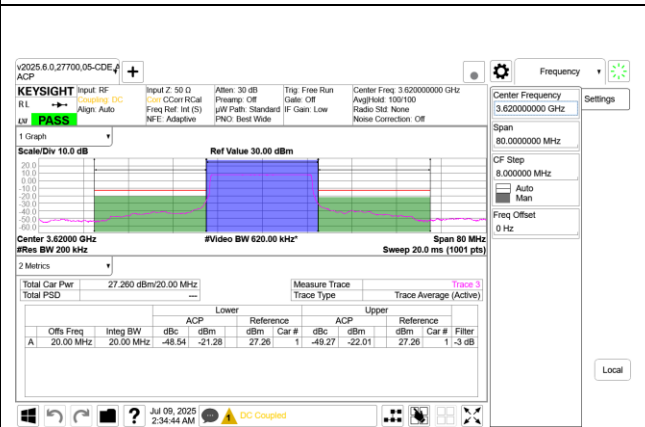
5G NR n48 20MHz BPSK Middle Channel RB50-0 Ant 9+8
