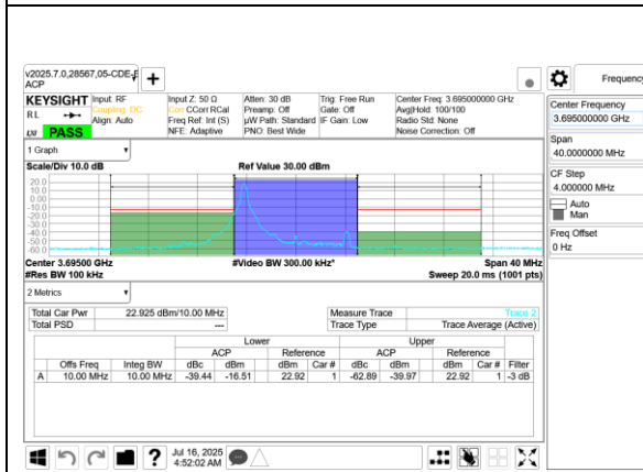
5G NR n48 10MHz BPSK High Channel RB1-0 Ant 8
