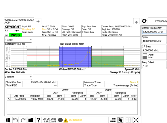
5G NR n48 10MHz BPSK Middle Channel RB1-23 Ant 9
