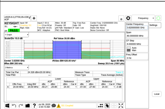
5G NR n48 20MHz BPSK Middle Channel RB50-0 Ant 8
