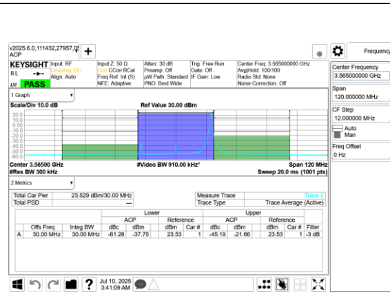
5G NR n48 30MHz BPSK Low Channel RB1-77 Ant 8
