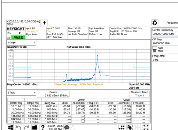
5G NR n48 20MHz QPSK Middle Channel RB1-50 Ant 9+8
