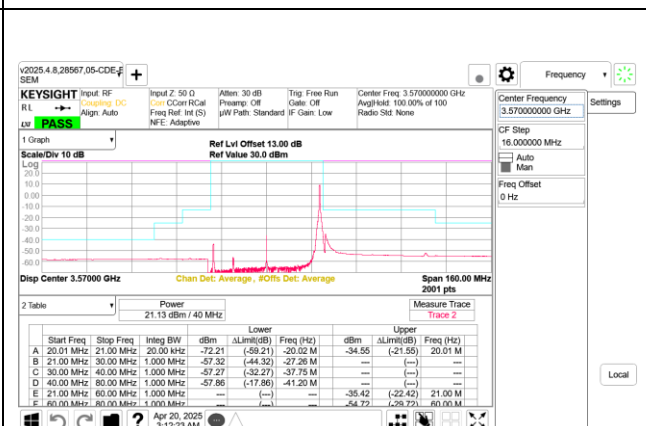
5G NR n48 40MHz QPSK Low Channel RB1-105 Ant 8
