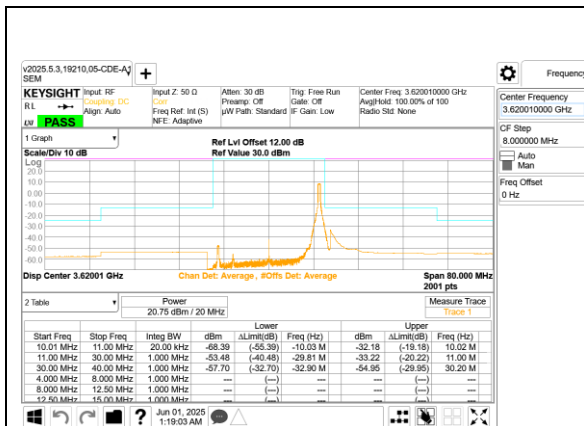
5G NR n48 20MHz QPSK Middle Channel RB1-50 Ant 9
