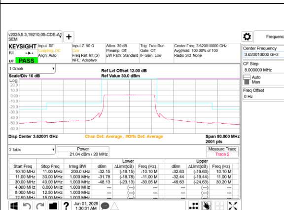
5G NR n48 20MHz QPSK Middle Channel RB51-0 Ant 8
