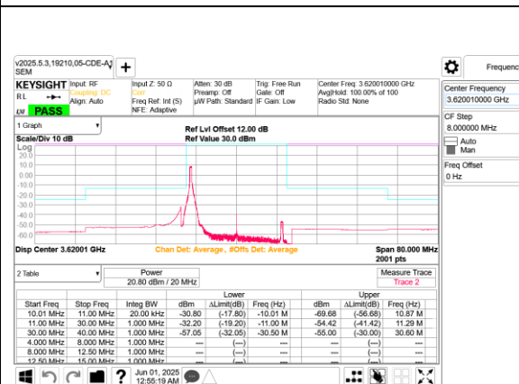
5G NR n48 20MHz QPSK Middle Channel RB1-0 Ant 8
