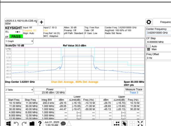
5G NR n48 20MHz QPSK Middle Channel RB51-0 Ant 9+8
