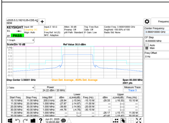
5G NR n48 20MHz QPSK Low Channel RB51-0 Ant 9+8
