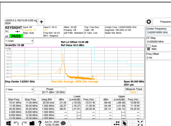
5G NR n48 20MHz QPSK Middle Channel RB1-0 Ant 9
