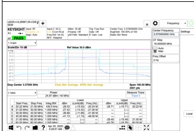
5G NR n48 40MHz QPSK Low Channel RB100-0 Ant 9+8
