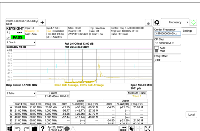
5G NR n48 40MHz QPSK Low Channel RB1-105 Ant 9
