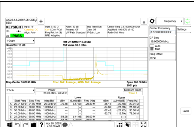
5G NR n48 40MHz QPSK High Channel RB1-105 Ant 9
