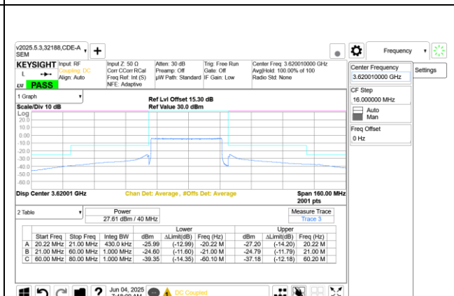
5G NR n48 40MHz QPSK Mid Channel RB100-0 Ant 9+8
