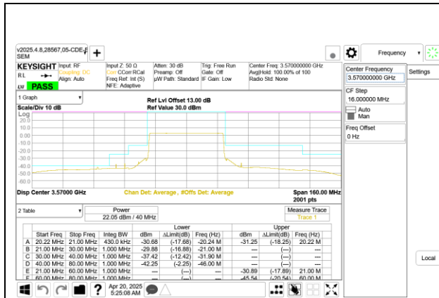
5G NR n48 40MHz QPSK Low Channel RB100-0 Ant 9
