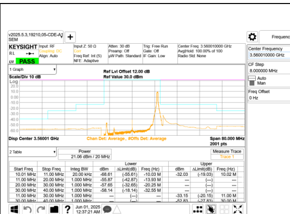
5G NR n48 20MHz QPSK Low Channel RB1-50 Ant 9
