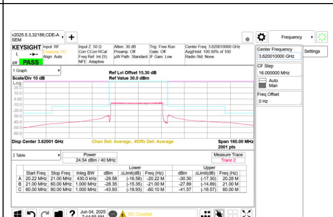
5G NR n48 40MHz QPSK Mid Channel RB100-0 Ant 8
