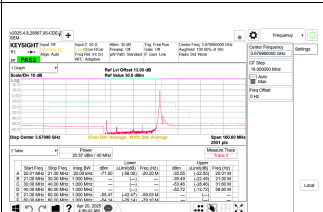
5G NR n48 40MHz QPSK High Channel RB1-105 Ant 8
