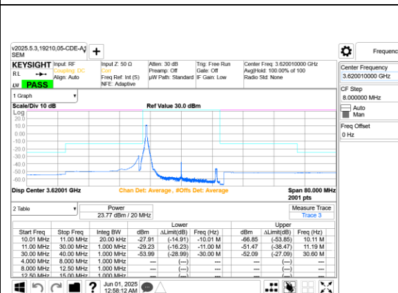
5G NR n48 20MHz QPSK Middle Channel RB1-0 Ant 9+8
