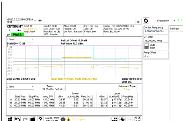
5G NR n48 40MHz QPSK Mid Channel RB100-0 Ant 9
