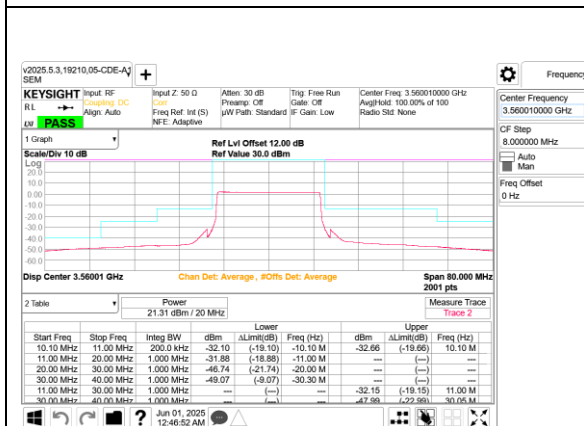
5G NR n48 20MHz QPSK Low Channel RB51-0 Ant 8
