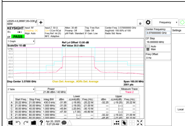
5G NR n48 40MHz QPSK Low Channel RB100-0 Ant 8
