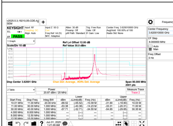
5G NR n48 20MHz QPSK Middle Channel RB1-50 Ant 8
