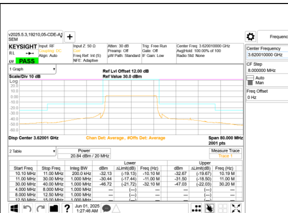
5G NR n48 20MHz QPSK Middle Channel RB51-0 Ant 9
