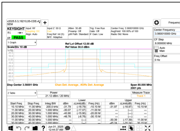
5G NR n48 20MHz QPSK Low Channel RB51-0 Ant 9
