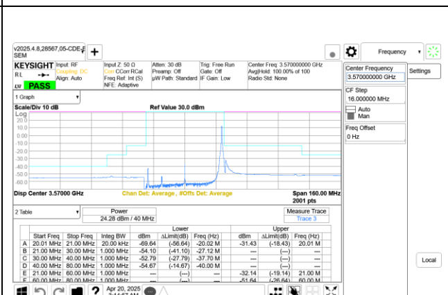
5G NR n48 40MHz QPSK Low Channel RB1-105 Ant 9+8
