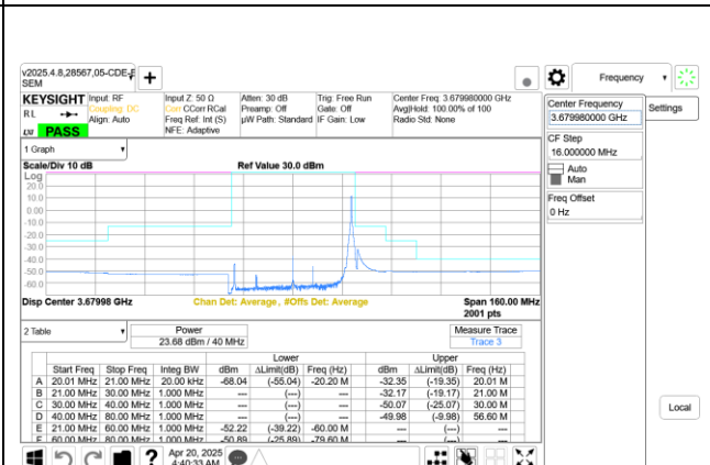
5G NR n48 40MHz QPSK High Channel RB1-105 Ant 9+8
