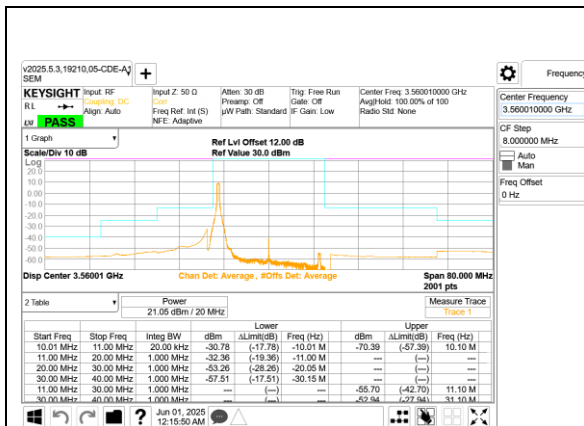
5G NR n48 20MHz QPSK Low Channel RB1-0 Ant 9
