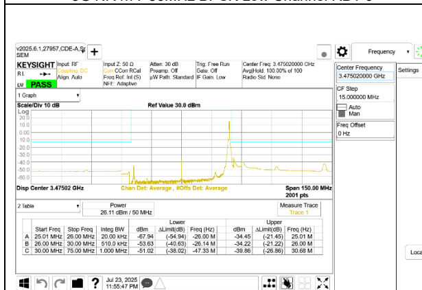
5G NR n77 50MHz BPSK Low Channel RB1-132
