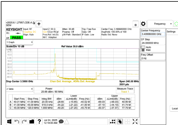
5G NR n77 80MHz BPSK Middle Channel RB1-0
