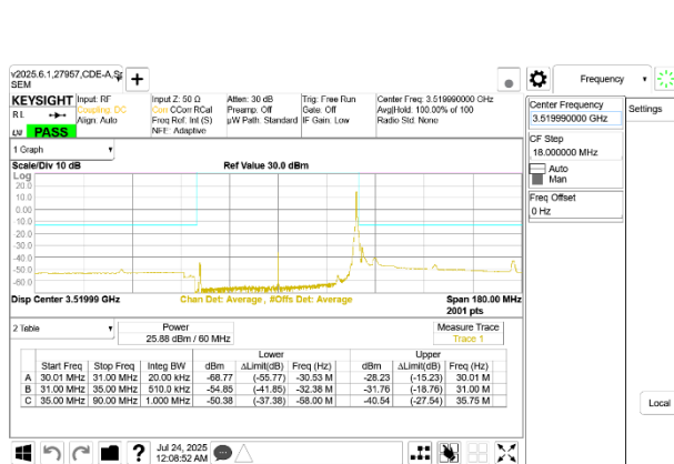
5G NR n77 60MHz BPSK High Channel RB1-161
