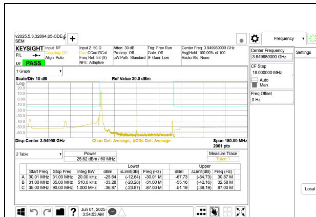
5G NR n77 60MHz BPSK High Channel RB1-0 Port A
