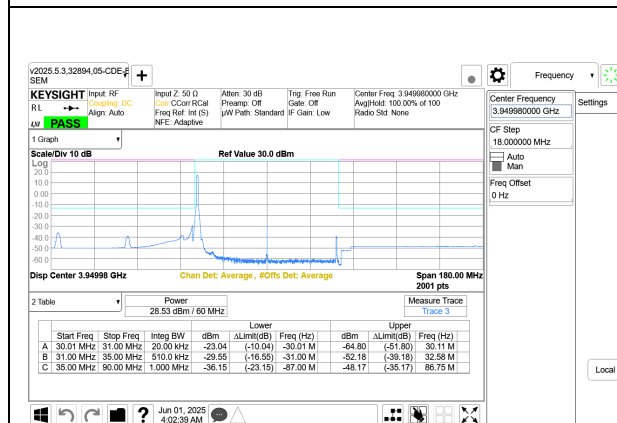
5G NR n77 60MHz BPSK High Channel RB1-0 Port A+B
