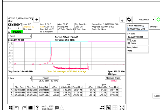
5G NR n77 60MHz BPSK High Channel RB1-0 Port B
