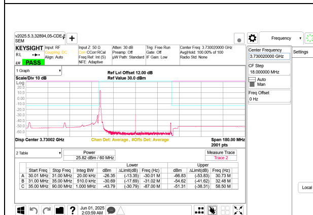
5G NR n77 60MHz BPSK Low Channel RB1-0 Port B
