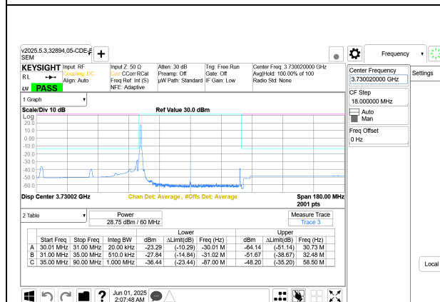
5G NR n77 60MHz BPSK Low Channel RB1-0 Port A+B
