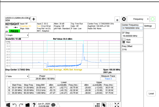
5G NR n77 60MHz BPSK Low Channel RB1-161 Port A+B
