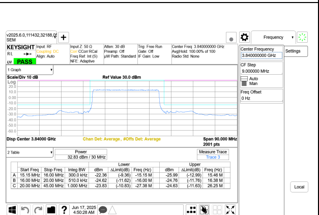
5G NR n77 30MHz BPSK Mid Channel RB75-0 Port A+B
