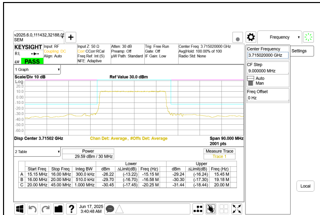
5G NR n77 30MHz BPSK Low Channel RB75-0 Port A
