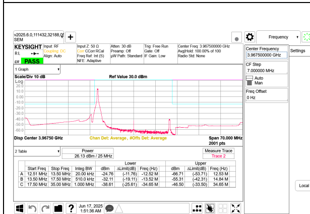
5G NR n77 25MHz BPSK High Channel RB1-0 Port B
