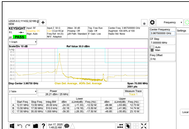
5G NR n77 25MHz BPSK High Channel RB1-0 Port A
