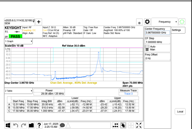
5G NR n77 25MHz BPSK High Channel RB1-64 Port A+B
