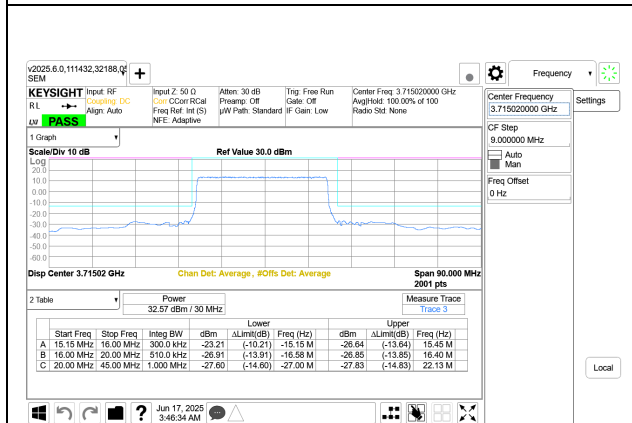
5G NR n77 30MHz BPSK Low Channel RB75-0 Port A+B
