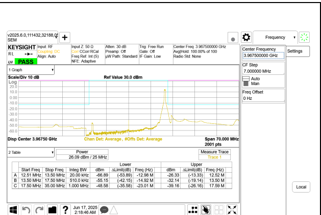
5G NR n77 25MHz BPSK High Channel RB1-64 Port A
