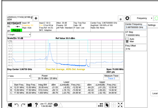
5G NR n77 25MHz BPSK High Channel RB1-0 Port A+B
