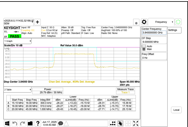
5G NR n77 30MHz BPSK Mid Channel RB75-0 Port A
