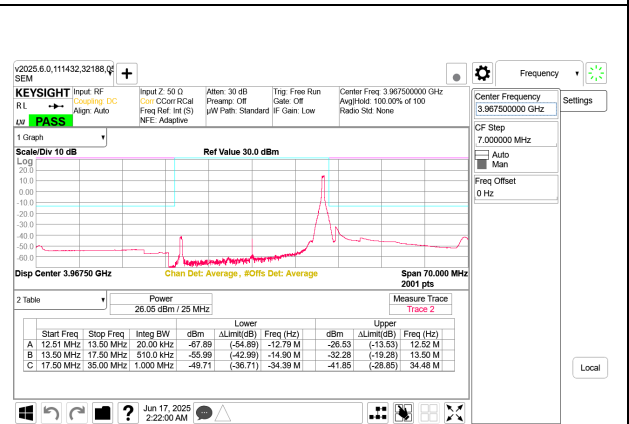
5G NR n77 25MHz BPSK High Channel RB1-64 Port B
