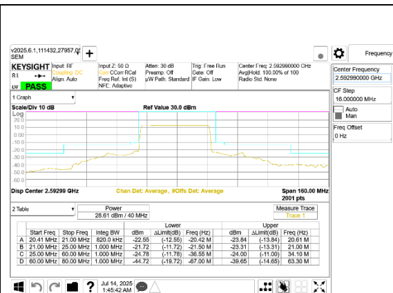
5G NR n41 40MHz BPSK Mid Channel RB100-0 Port A
