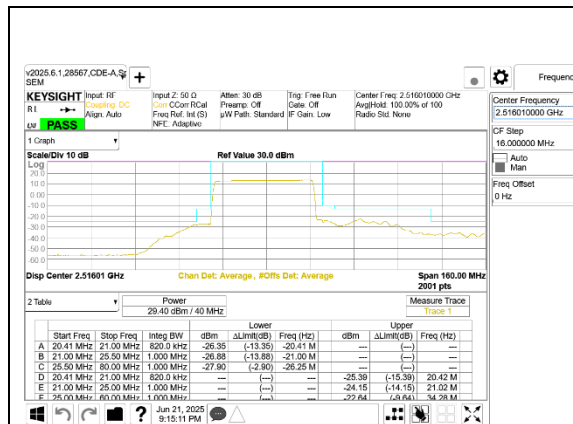
5G NR n41 40MHz BPSK Low Channel RB100-0 Port A
