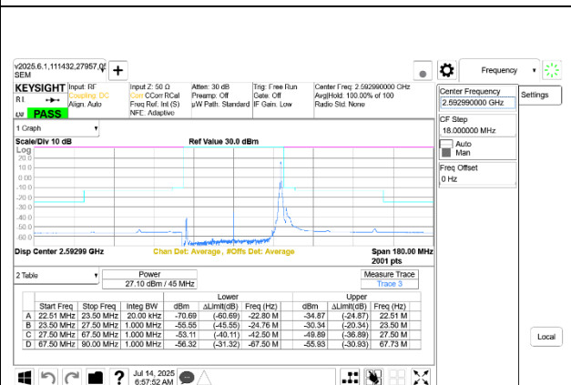
5G NR n41 45MHz BPSK Mid Channel RB1-118 Port A+B
