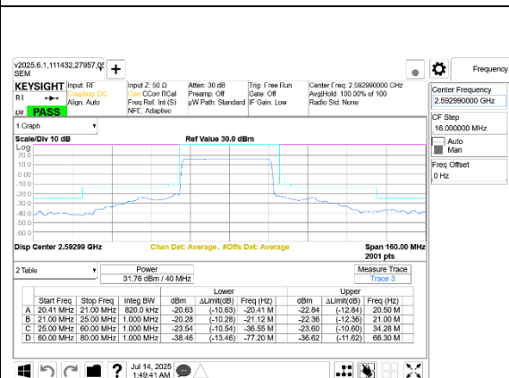
5G NR n41 40MHz BPSK Mid Channel RB100-0 Port A+B
