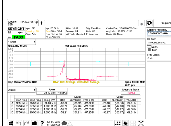
5G NR n41 45MHz BPSK Middle Channel RB1-0 Port B
