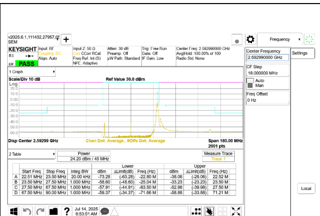
5G NR n41 45MHz BPSK Mid Channel RB1-118 Port A
