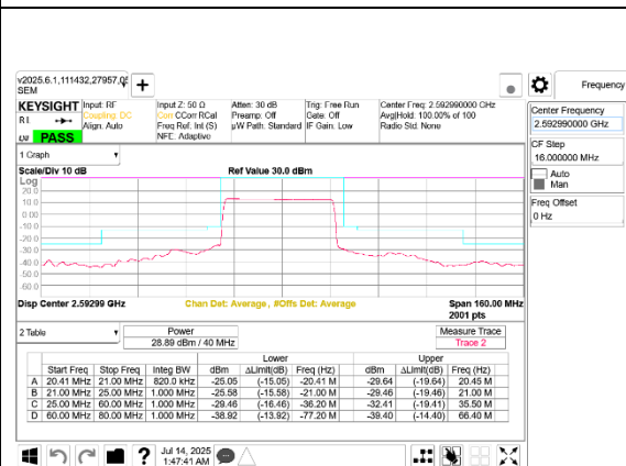
5G NR n41 40MHz BPSK Mid Channel RB100-0 Port B
