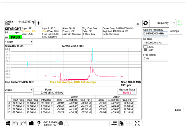
5G NR n41 45MHz BPSK Mid Channel RB1-118 Port B
