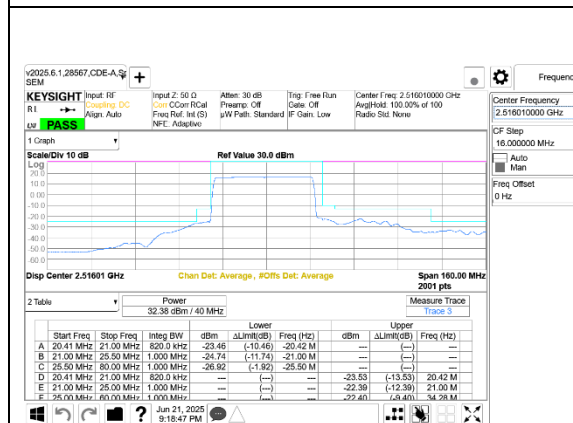
5G NR n41 40MHz BPSK Low Channel RB100-0 Port A+B
