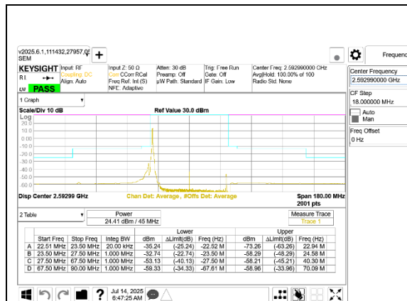
5G NR n41 45MHz BPSK Middle Channel RB1-0 Port A
