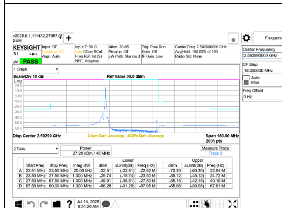
5G NR n41 45MHz BPSK Middle Channel RB1-0 Port A+B
