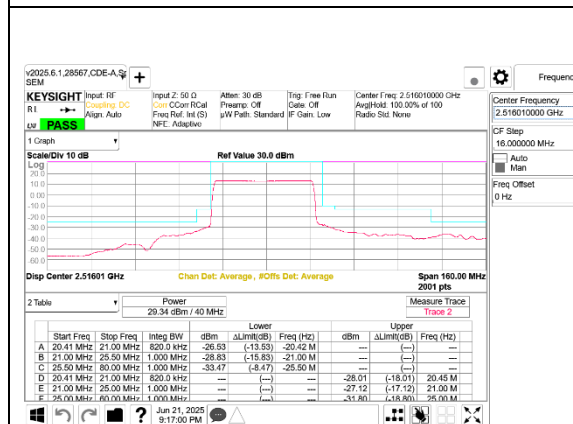
5G NR n41 40MHz BPSK Low Channel RB100-0 Port B
