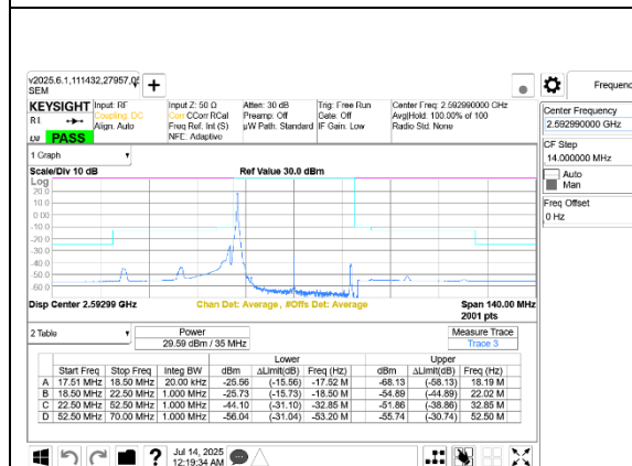
5G NR n41 35MHz BPSK Middle Channel RB1-0 Port A+B
