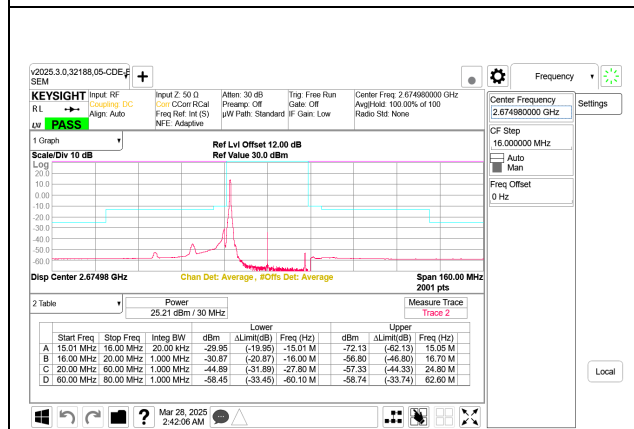
5G NR n41 30MHz BPSK High Channel RB1-0 Port B
