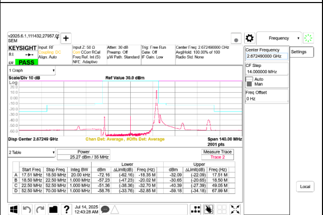
5G NR n41 35MHz BPSK High Channel RB1-91 Port B
