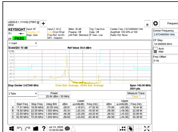
5G NR n41 35MHz BPSK High Channel RB1-0 Port A
