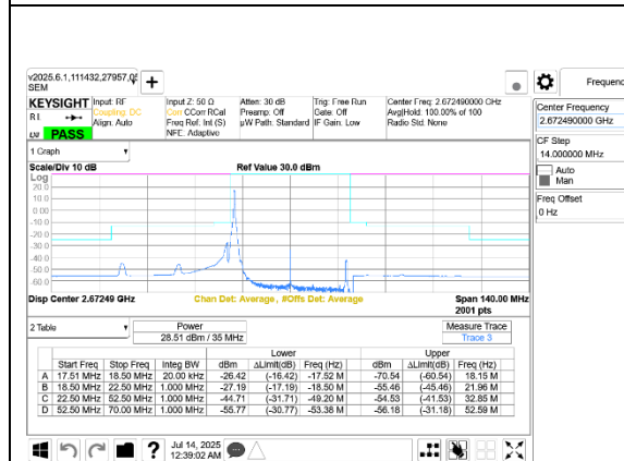
5G NR n41 35MHz BPSK High Channel RB1-0 Port A+B
