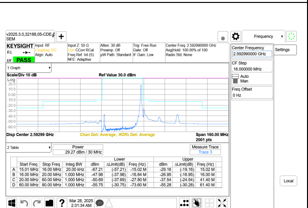
5G NR n41 30MHz BPSK Mid Channel RB1-77 Port A+B
