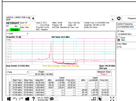
5G NR n41 35MHz BPSK Low Channel RB1-0 Port B
