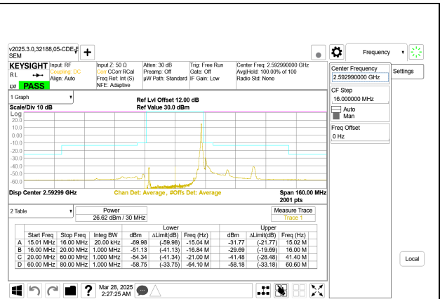
5G NR n41 30MHz BPSK Mid Channel RB1-77 Port A
