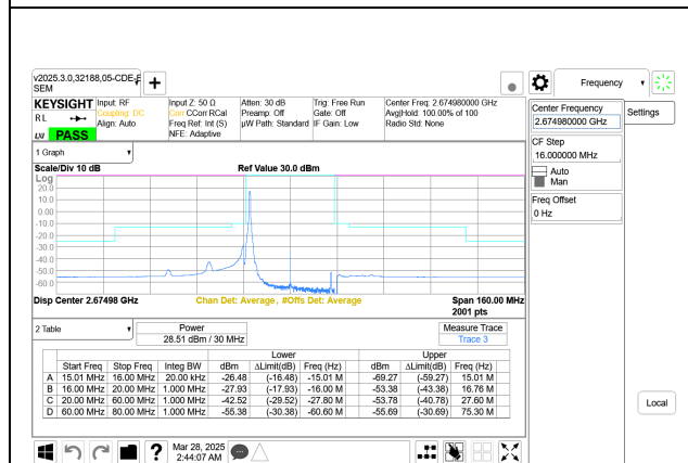
5G NR n41 30MHz BPSK High Channel RB1-0 Port A+B
