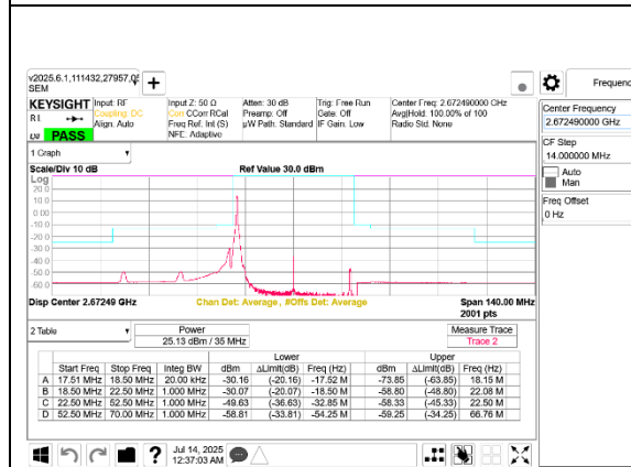
5G NR n41 35MHz BPSK High Channel RB1-0 Port B
