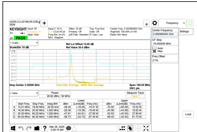
5G NR n41 30MHz BPSK Middle Channel RB1-0 Port A
