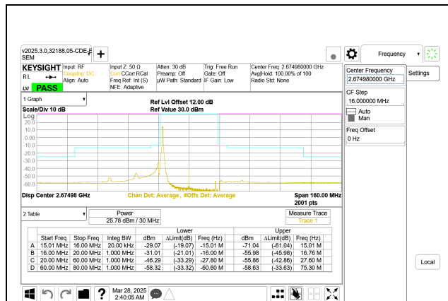
5G NR n41 30MHz BPSK High Channel RB1-0 Port A
