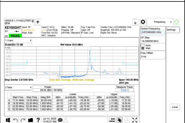
5G NR n41 35MHz BPSK High Channel RB1-91 Port A+B
