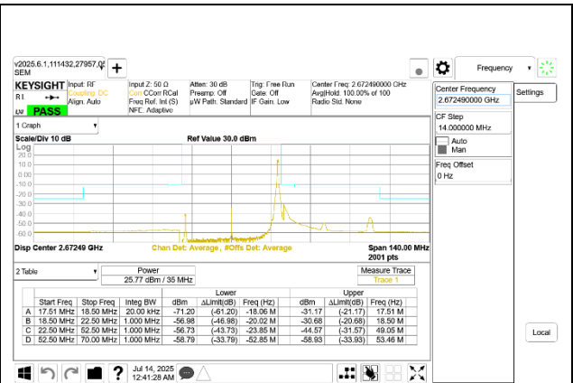
5G NR n41 35MHz BPSK High Channel RB1-91 Port A
