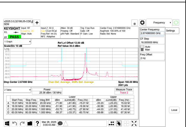
5G NR n41 30MHz BPSK High Channel RB1-77 Port B
