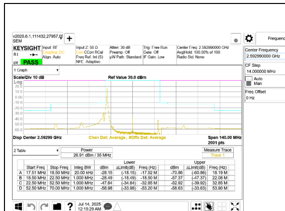
5G NR n41 35MHz BPSK Middle Channel RB1-0 Port A
