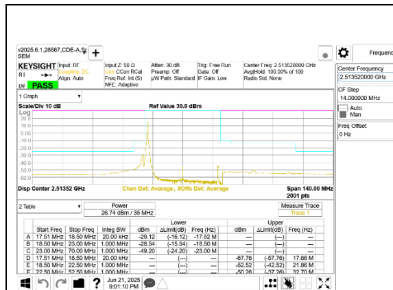
5G NR n41 35MHz BPSK Low Channel RB1-0 Port A
