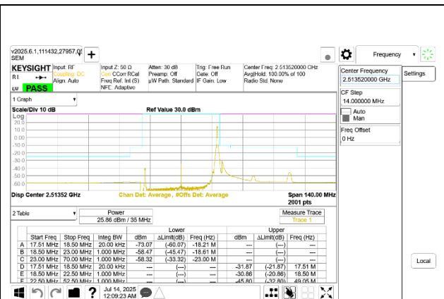
5G NR n41 35MHz BPSK Low Channel RB1-91 Port A
