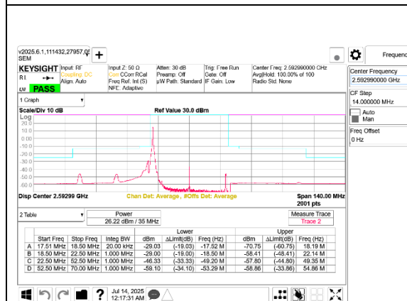
5G NR n41 35MHz BPSK Middle Channel RB1-0 Port B
