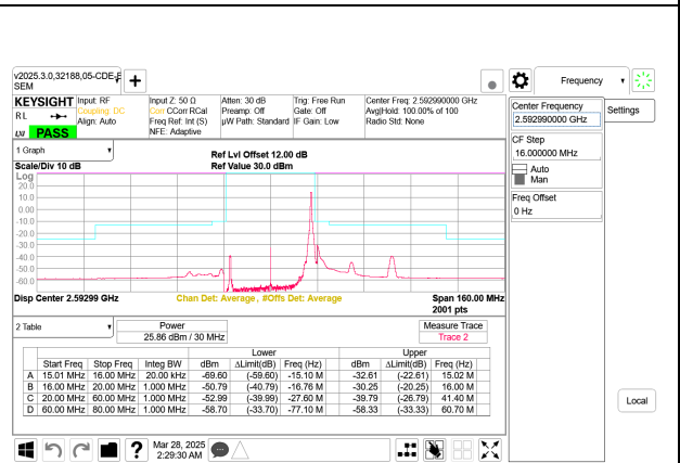
5G NR n41 30MHz BPSK Mid Channel RB1-77 Port B
