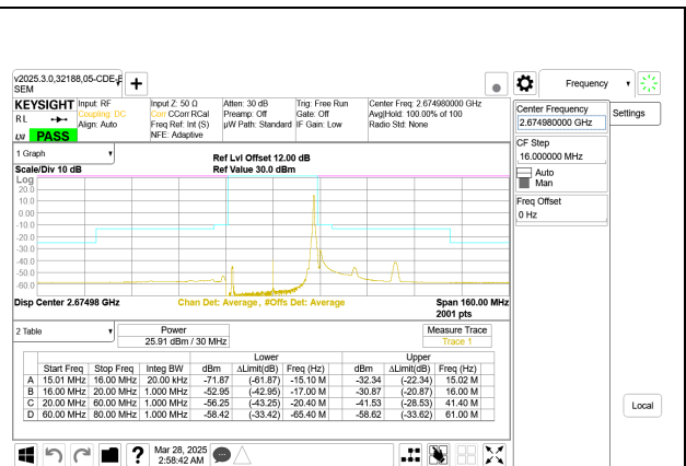
5G NR n41 30MHz BPSK High Channel RB1-77 Port A
