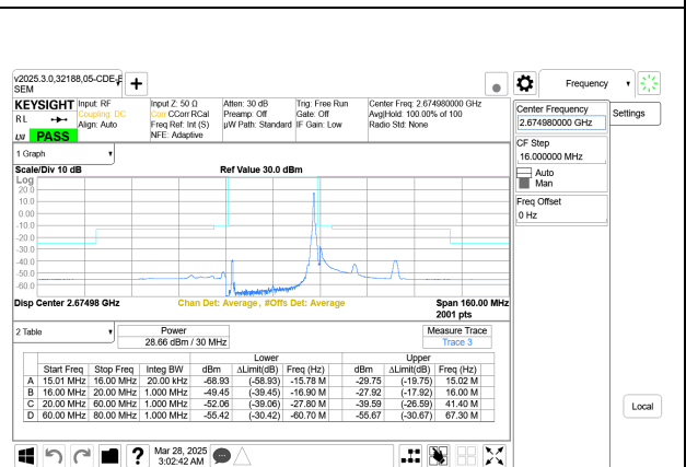
5G NR n41 30MHz BPSK High Channel RB1-77 Port A+B
