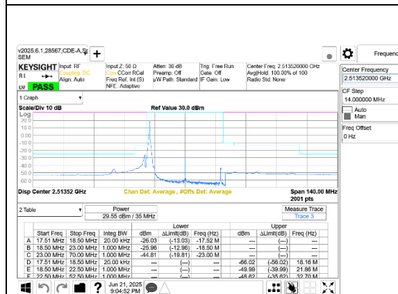
5G NR n41 35MHz BPSK Low Channel RB1-0 Port A+B
