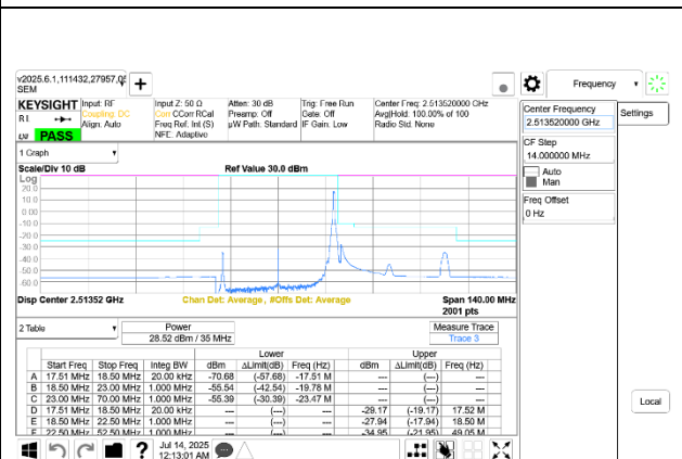
5G NR n41 35MHz BPSK Low Channel RB1-91 Port A+B
