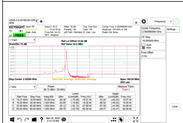
5G NR n41 30MHz BPSK Middle Channel RB1-0 Port B
