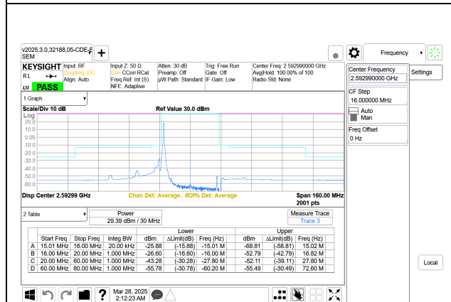
5G NR n41 30MHz BPSK Middle Channel RB1-0 Port A+B
