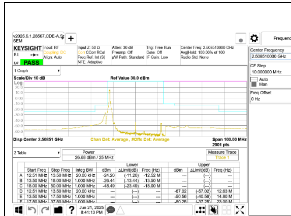
5G NR n41 25MHz BPSK Low Channel RB1-0 Port A
