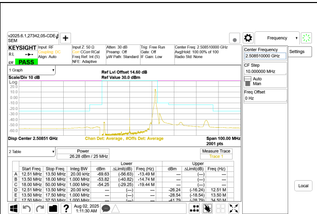
5G NR n41 25MHz BPSK Low Channel RB1-64 Port A
