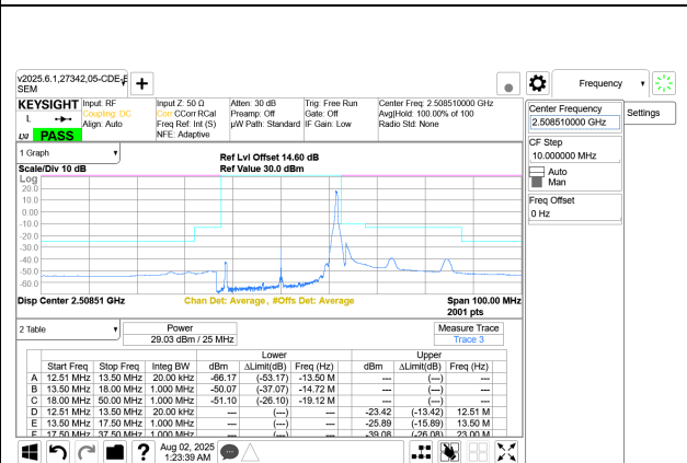
5G NR n41 25MHz BPSK Low Channel RB1-64 Port A+B
