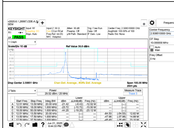
5G NR n41 25MHz BPSK Low Channel RB1-0 Port A+B
