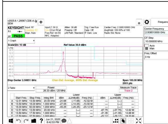
5G NR n41 25MHz BPSK Low Channel RB1-0 Port B
