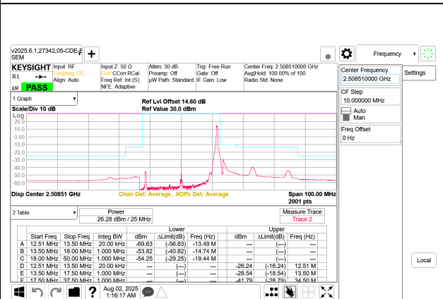
5G NR n41 25MHz BPSK Low Channel RB1-64 Port B
