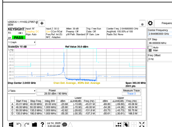
5G NR n41 90MHz BPSK High Channel RB1-0 Port A+B
