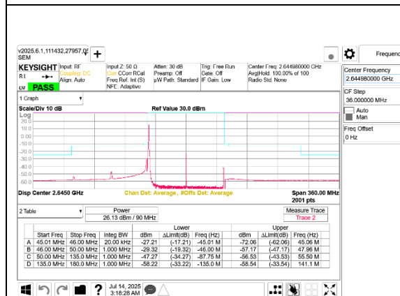
5G NR n41 90MHz BPSK High Channel RB1-0 Port B
