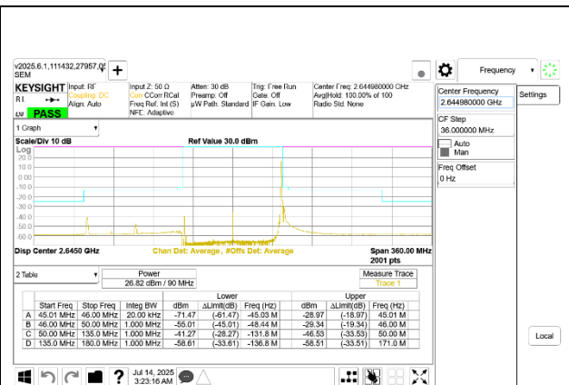
5G NR n41 90MHz BPSK High Channel RB1-244 Port A
