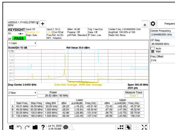
5G NR n41 90MHz BPSK High Channel RB1-0 Port A
