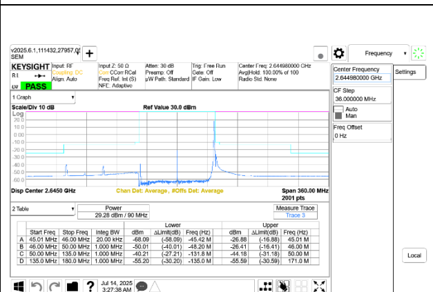
5G NR n41 90MHz BPSK High Channel RB1-244 Port A+B
