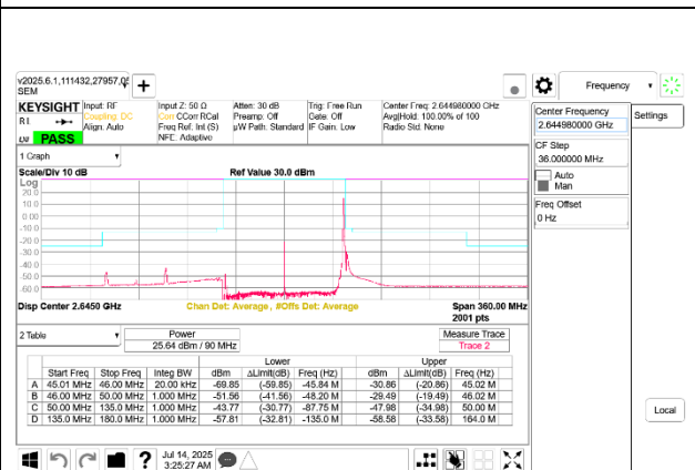
5G NR n41 90MHz BPSK High Channel RB1-244 Port B
