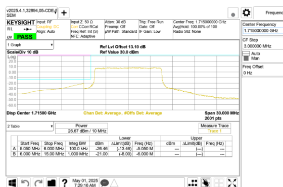
LTE B66 10MHz QPSK Low Channel RB50-0
