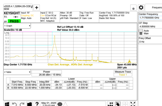
LTE B66 15MHz QPSK Low Channel RB1-0
