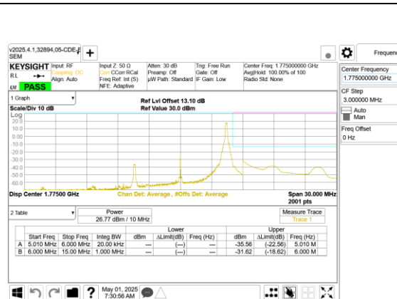
LTE B66 10MHz QPSK High Channel RB1-49
