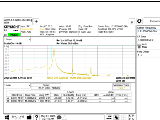
LTE B66 10MHz QPSK Low Channel RB1-0
