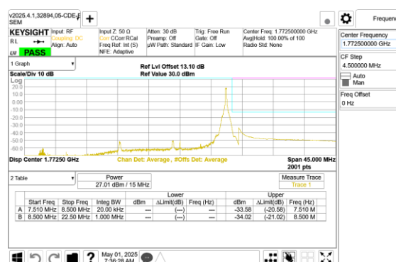
LTE B66 15MHz QPSK High Channel RB1-74
