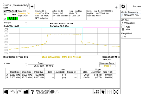
LTE B66 10MHz QPSK High Channel RB50-0
