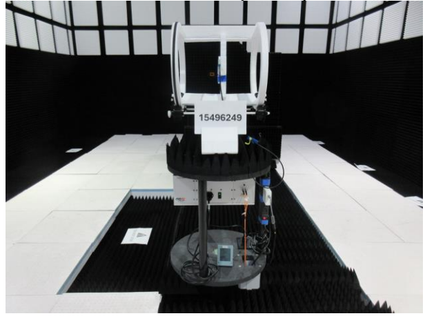
50 - 75 GHz (BACK)
