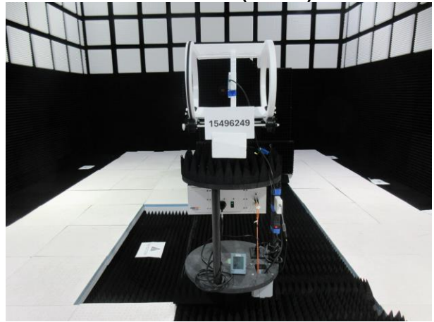
50 - 75 GHz (BACK)
