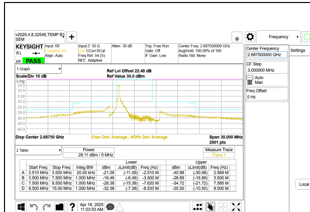
LTE B41 5MHz QPSK High Channel RB1-0
