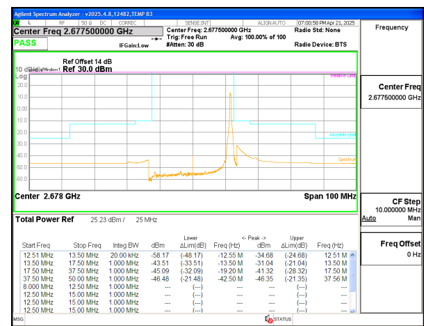
5G NR n41 25MHz BPSK High Channel RB1-64
