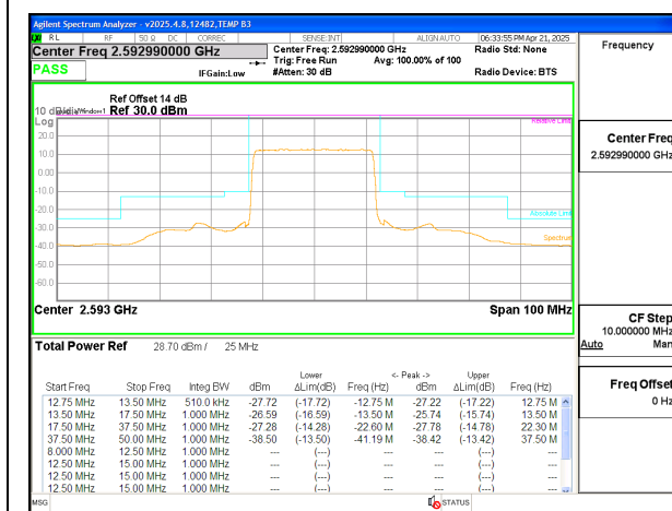
5G NR n41 25MHz BPSK Middle Channel RB64-0
