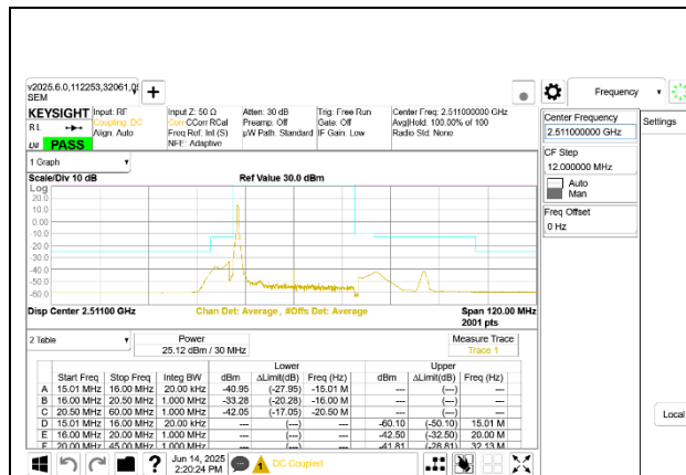
5G NR n41 30MHz BPSK Low Channel RB1-0
