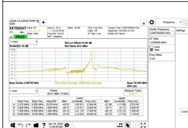
LTE B41 5MHz QPSK High Channel RB1-24
