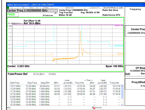
5G NR n41 25MHz BPSK Middle Channel RB1-64
