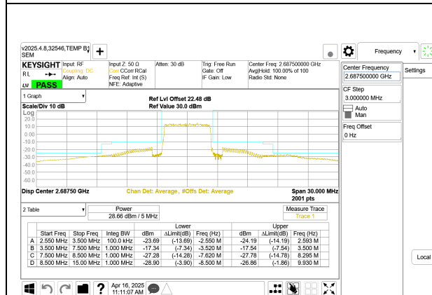
LTE B41 5MHz QPSK High Channel RB25-0
