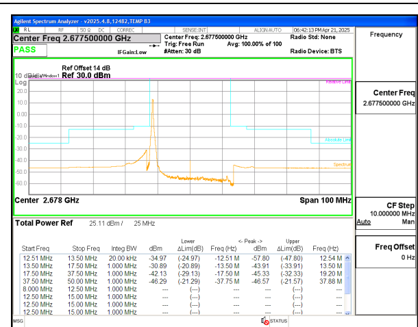
5G NR n41 25MHz BPSK High Channel RB1-0
