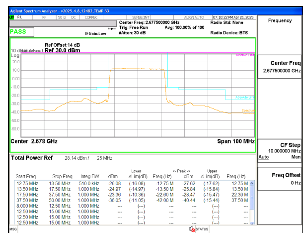
5G NR n41 25MHz BPSK High Channel RB64-0
