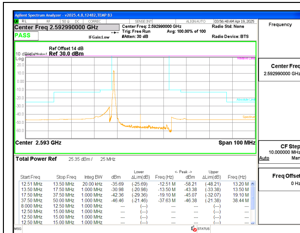
5G NR n41 25MHz BPSK Middle Channel RB1-0
