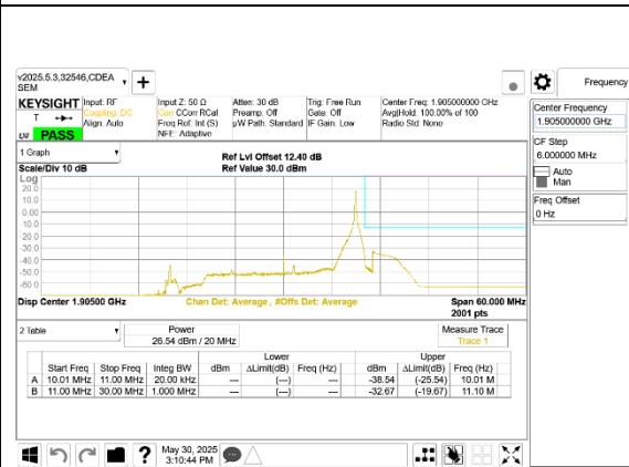
LTE B25 20MHz QPSK High Channel RB1-99
