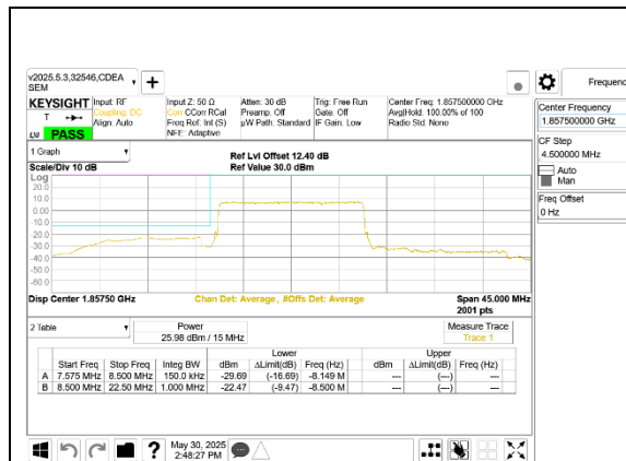
LTE B25 15MHz QPSK Low Channel RB75-0
