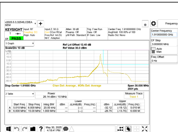
LTE B25 10MHz QPSK High Channel RB1-49
