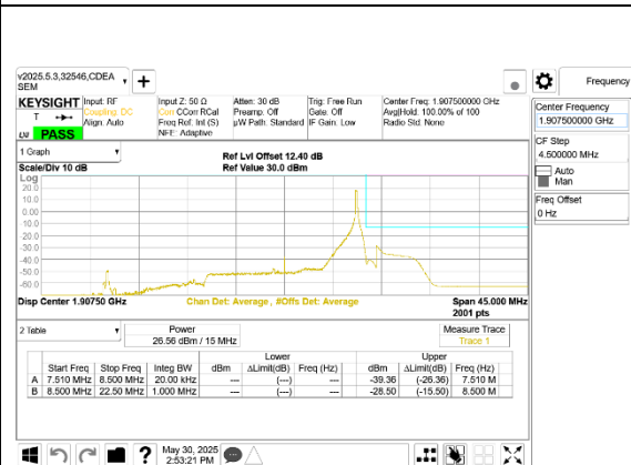
LTE B25 15MHz QPSK High Channel RB1-74
