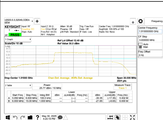
LTE B25 10MHz QPSK High Channel RB50-0
