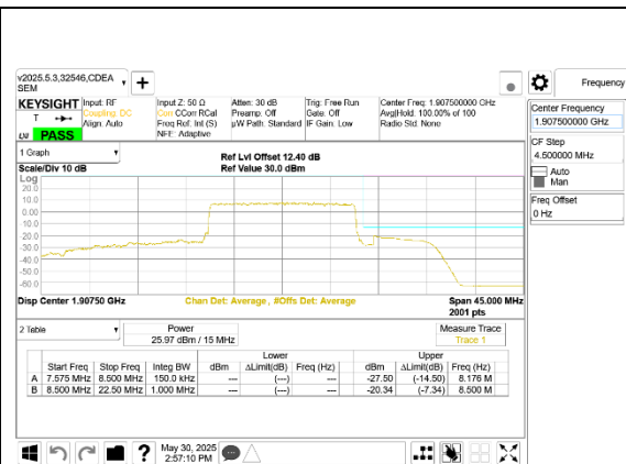
LTE B25 15MHz QPSK High Channel RB75-0
