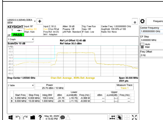
LTE B25 10MHz QPSK Low Channel RB50-0
