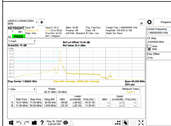
LTE B25 20MHz QPSK Low Channel RB1-0
