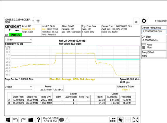
LTE B25 20MHz QPSK High Channel RB100-0
