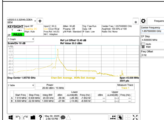
LTE B25 15MHz QPSK Low Channel RB1-0
