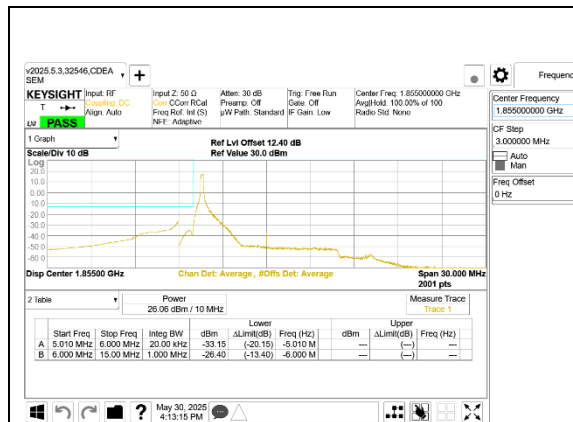
LTE B25 10MHz QPSK Low Channel RB1-0
