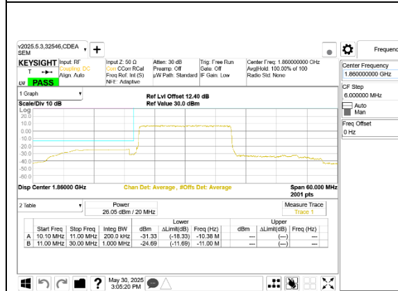
LTE B25 20MHz QPSK Low Channel RB100-0
