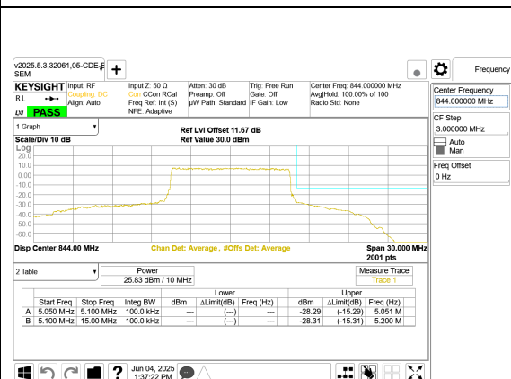
LTE B5 10MHz QPSK High Channel RB50-0
