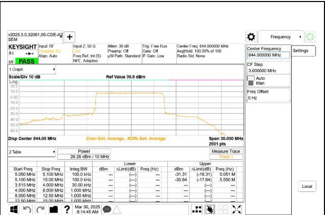
5G NR n5 10MHz BPSK High Channel RB50-0
