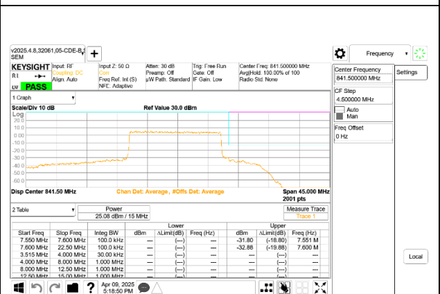
5G NR n5 15MHz BPSK High Channel RB75-0
