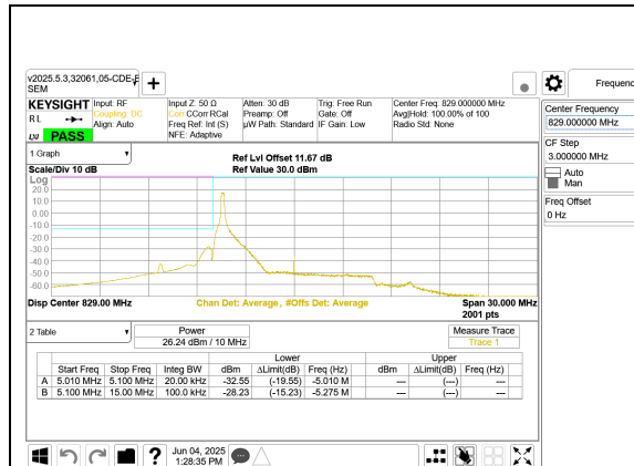
LTE B5 10MHz QPSK Low Channel RB1-0
