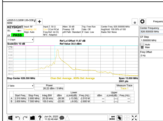
LTE B5 5MHz QPSK Low Channel RB1-0
