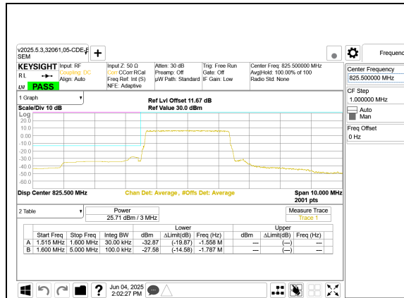
LTE B5 3MHz QPSK Low Channel RB15-0
