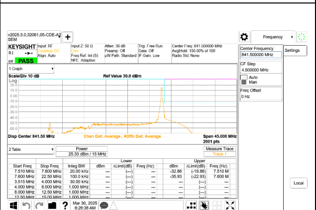
5G NR n5 15MHz BPSK High Channel RB1-78
