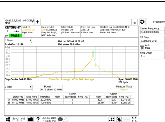
LTE B5 10MHz QPSK High Channel RB1-49
