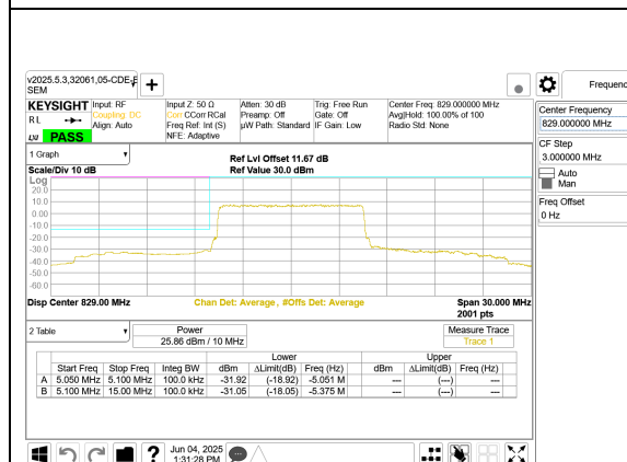
LTE B5 10MHz QPSK Low Channel RB50-0
